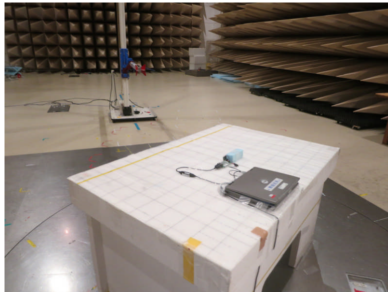
Photo2 Test setup for radiated
