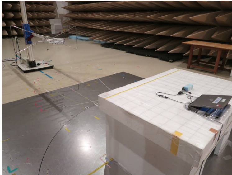
Photo3 Test setup for radiated
