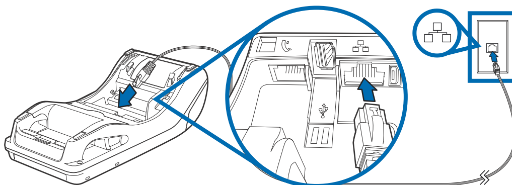
Figure 10 Ethernet Connection
