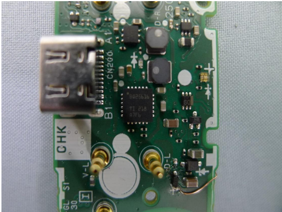
(21) EUT Photo (charging case)
