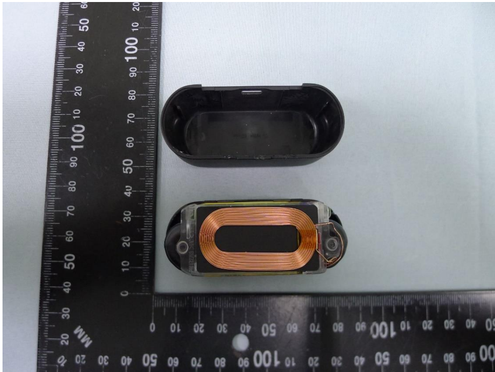
(14) EUT Photo (charging case)
