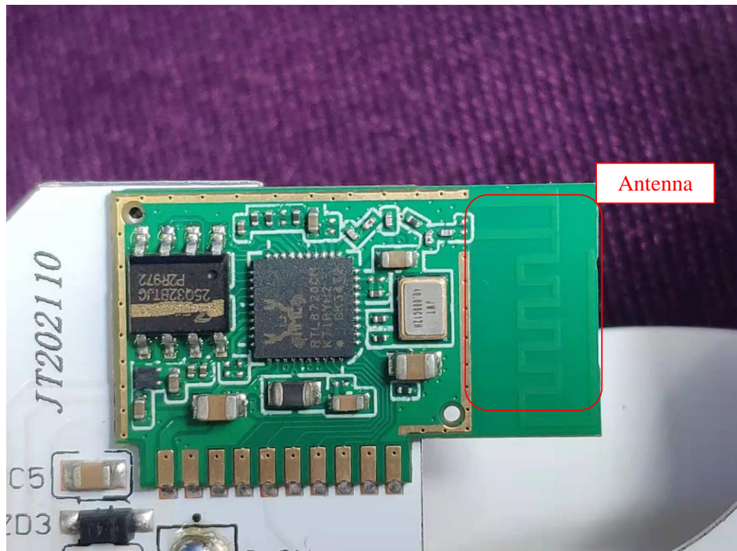
FIGURE 8 CYNCR FIXTURE CANLESS (M/N: CFIxCNLR4S1) POWER BOARD (COMPONENT SIDE)
