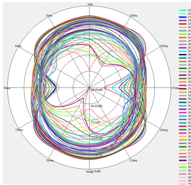
LTE B7/B38/B40/B41/B42 NR n7/n38/n40/n41/n77/n78 \Theta=90^\circ
