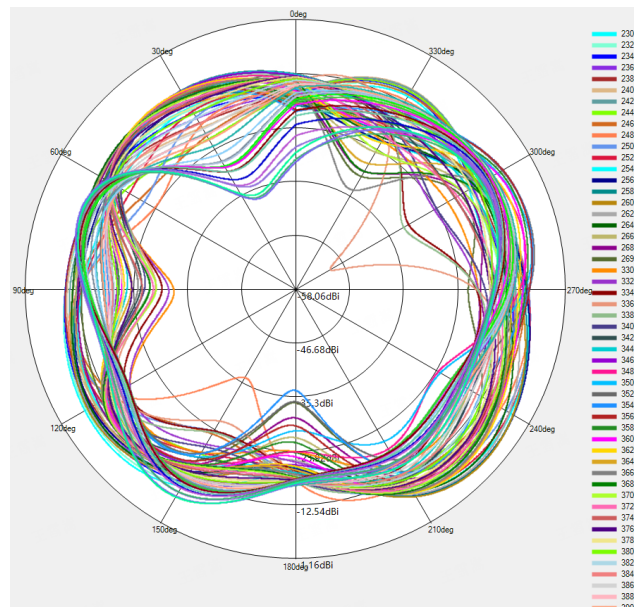
LTE B7/B38/B40/B41/B42 NR n7/n38/n40/n41/n77/n78 \Phi=90^\circ
