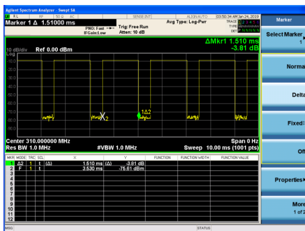
(Duty cycle 3) T_{ON(1 \text{ hop})}
