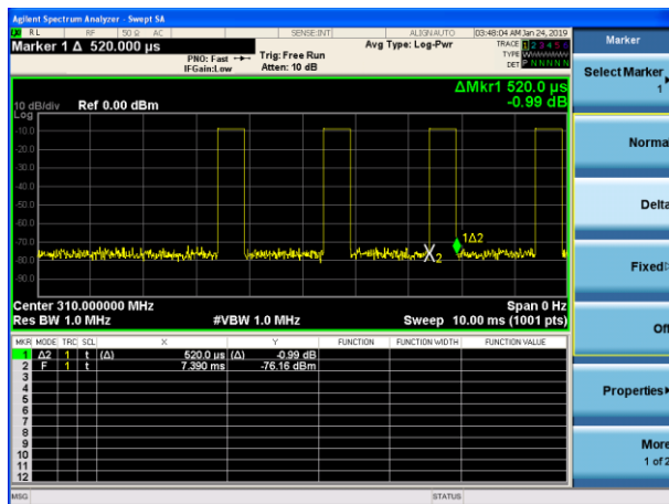
(Duty cycle 1) T_{ON(1 \text{ hop})}
