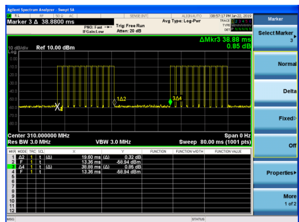
(Duty cycle 3) The duration of one cycle
