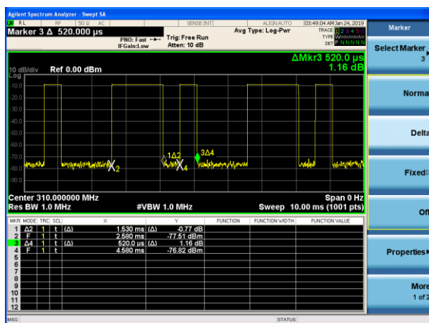
(Duty cycle 2) T_{ON(1 \text{ hop})}
