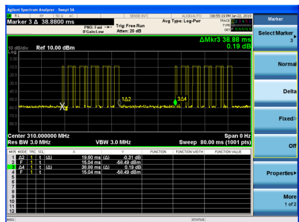
(Duty cycle 2) The duration of one cycle
