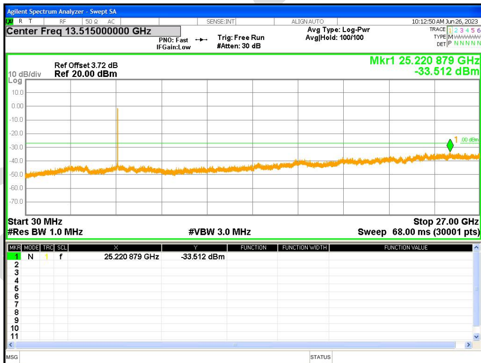
Tx. Spurious NVNT ac40 5570MHz Ant1 Emission
