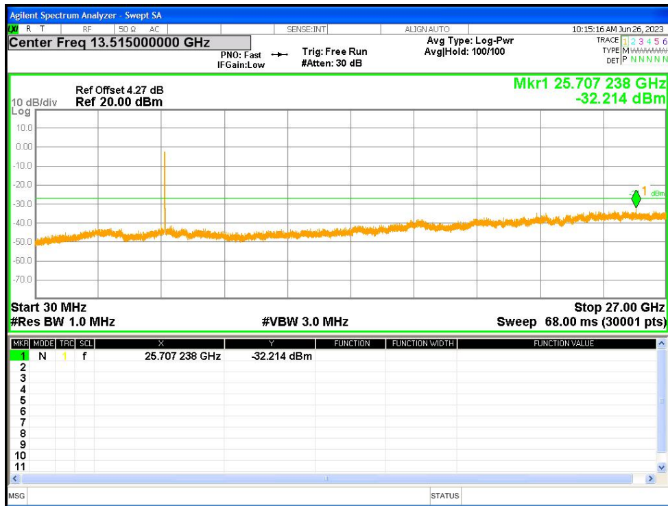
Tx. Spurious NVNT ac40 5570MHz Ant2 Emission
