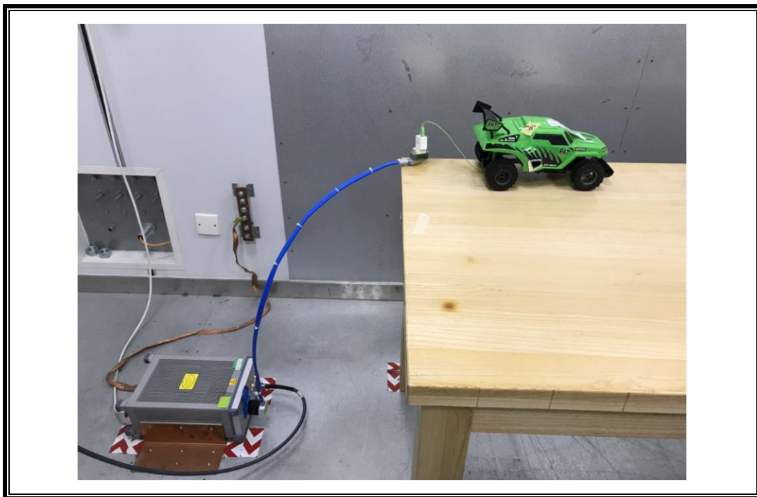
CONDUCTED EMISSION
