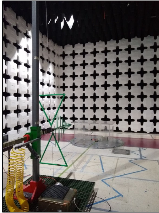
Photograph 1. Radiated Emissions, 30 MHz – 1 GHz, Test Setup
