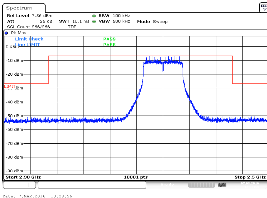
Plot 6: 2452 MHz, zoomed carrier
