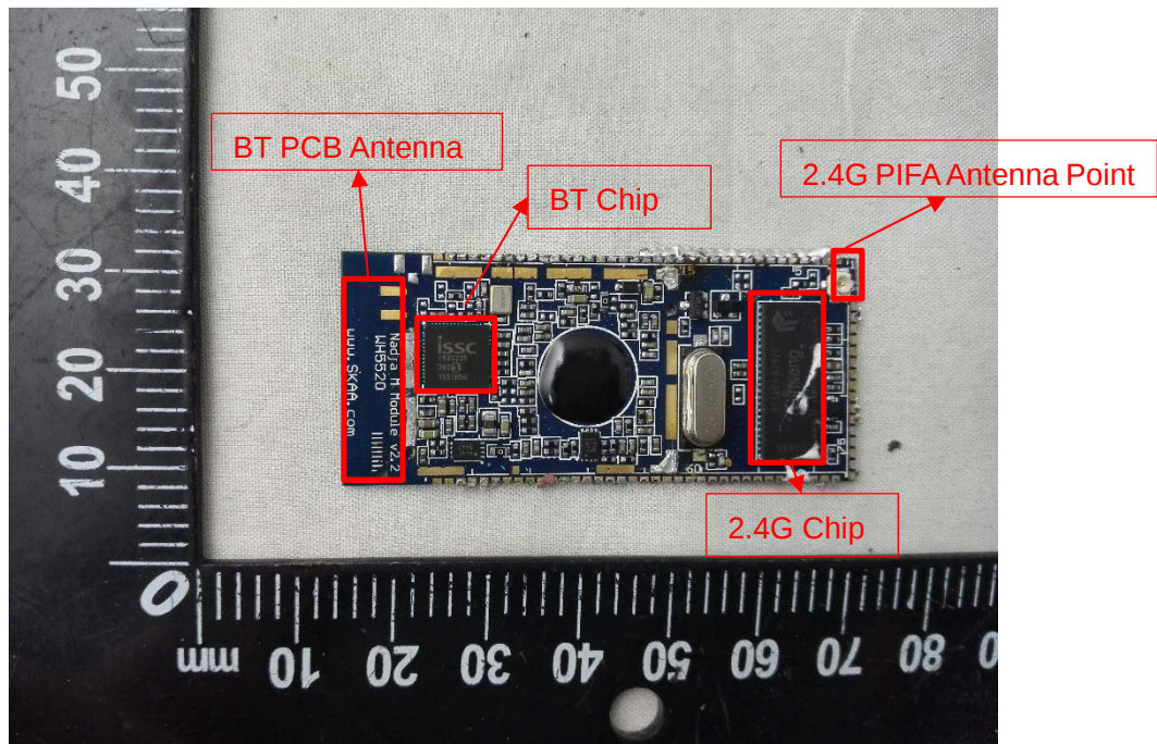
MAIN BOARD TOP VIEW 5
