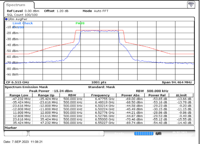
802.11ax-20 MHz / 6515 MHz / Chain B
