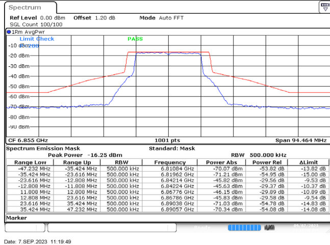
802.11ax-20 MHz / 6855 MHz / Chain A
