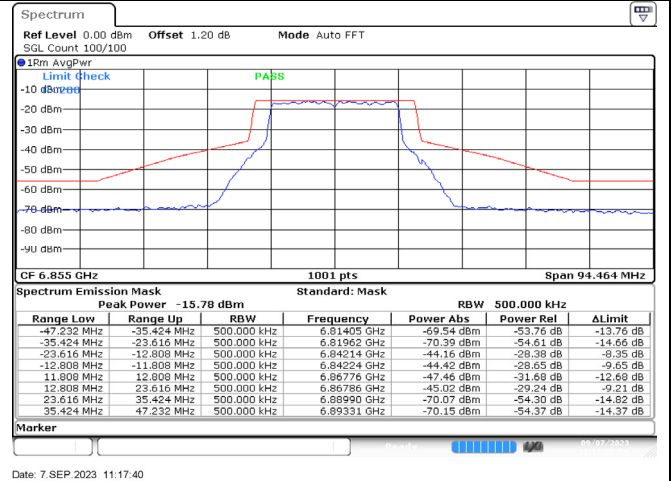
802.11ax-20 MHz / 6855 MHz / Chain B
