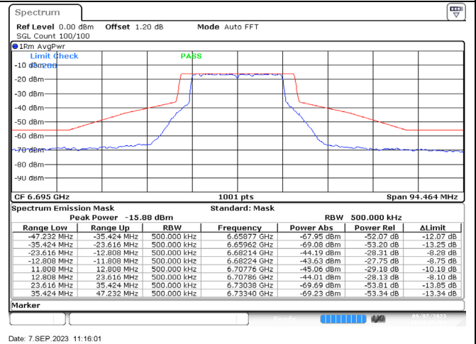
802.11ax-20 MHz / 6695 MHz / Chain B
