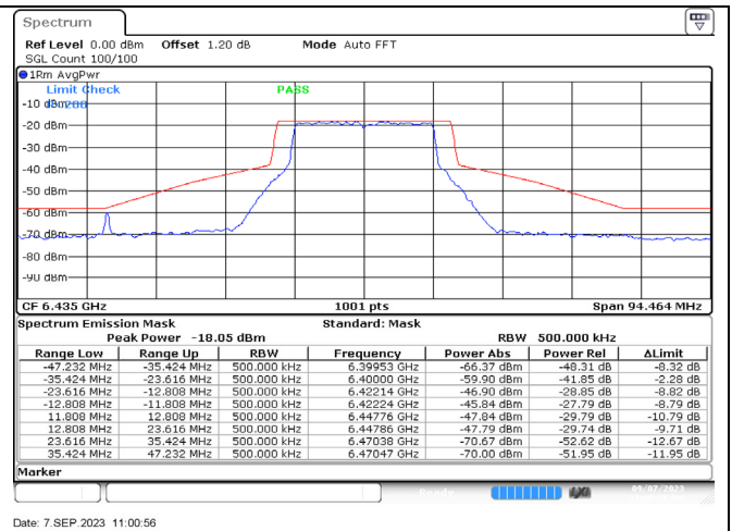
802.11ax-20 MHz / 6435 MHz / Chain B
