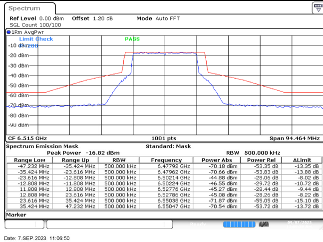
802.11ax-20 MHz / 6515 MHz / Chain A
