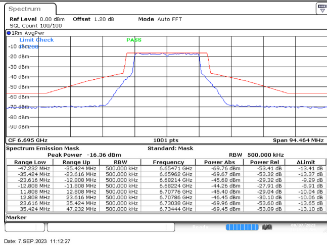
802.11ax-20 MHz / 6695 MHz / Chain A
