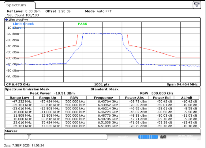
802.11ax-20 MHz / 6475 MHz / Chain B
