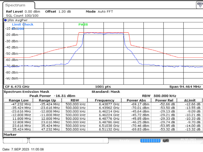
802.11ax-20 MHz / 6475 MHz / Chain A
