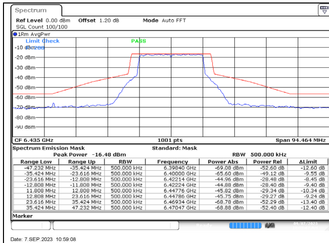
802.11ax-20 MHz / 6435 MHz / Chain A
