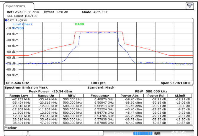
802.11ax-20 MHz / 6535 MHz / Chain B
