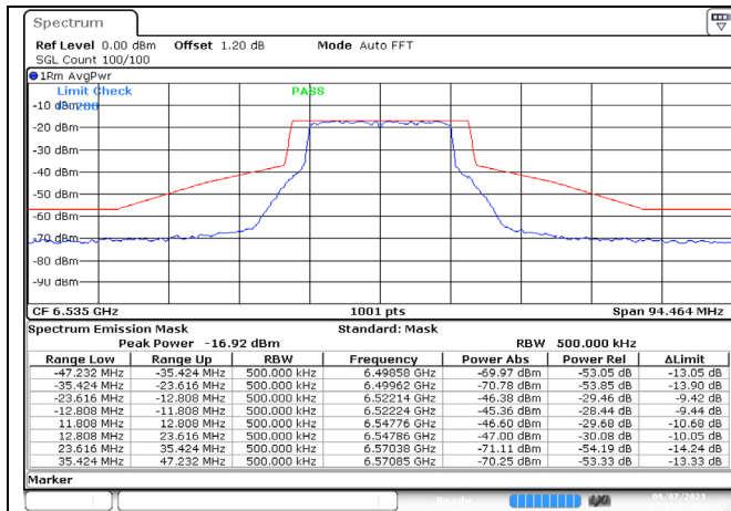
802.11ax-20 MHz / 6535 MHz / Chain A
