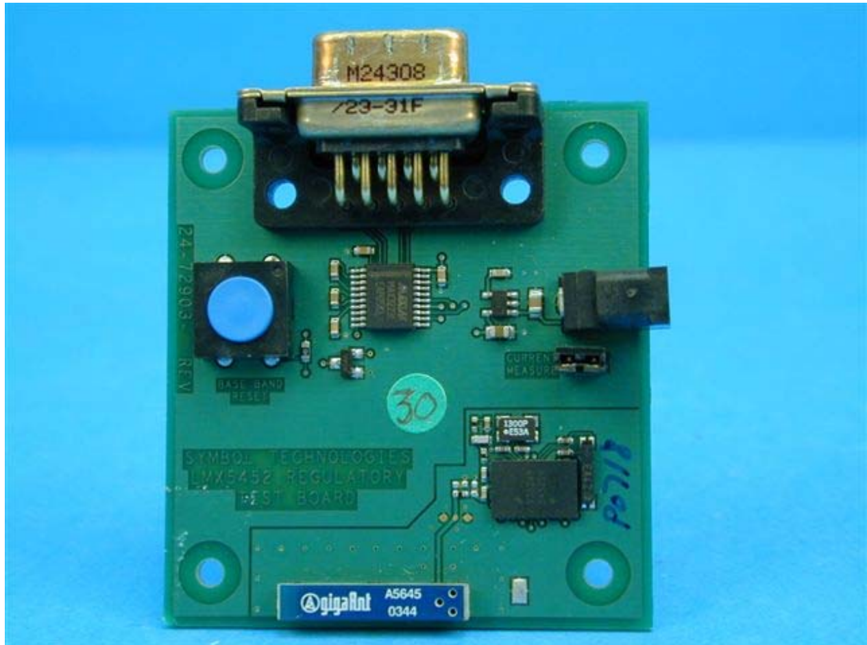
Front View
