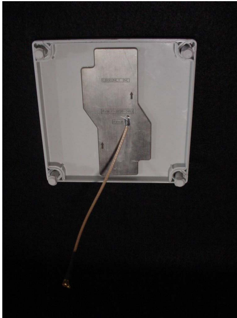
Figure 2: Rear side with rear enclosure cover removed
