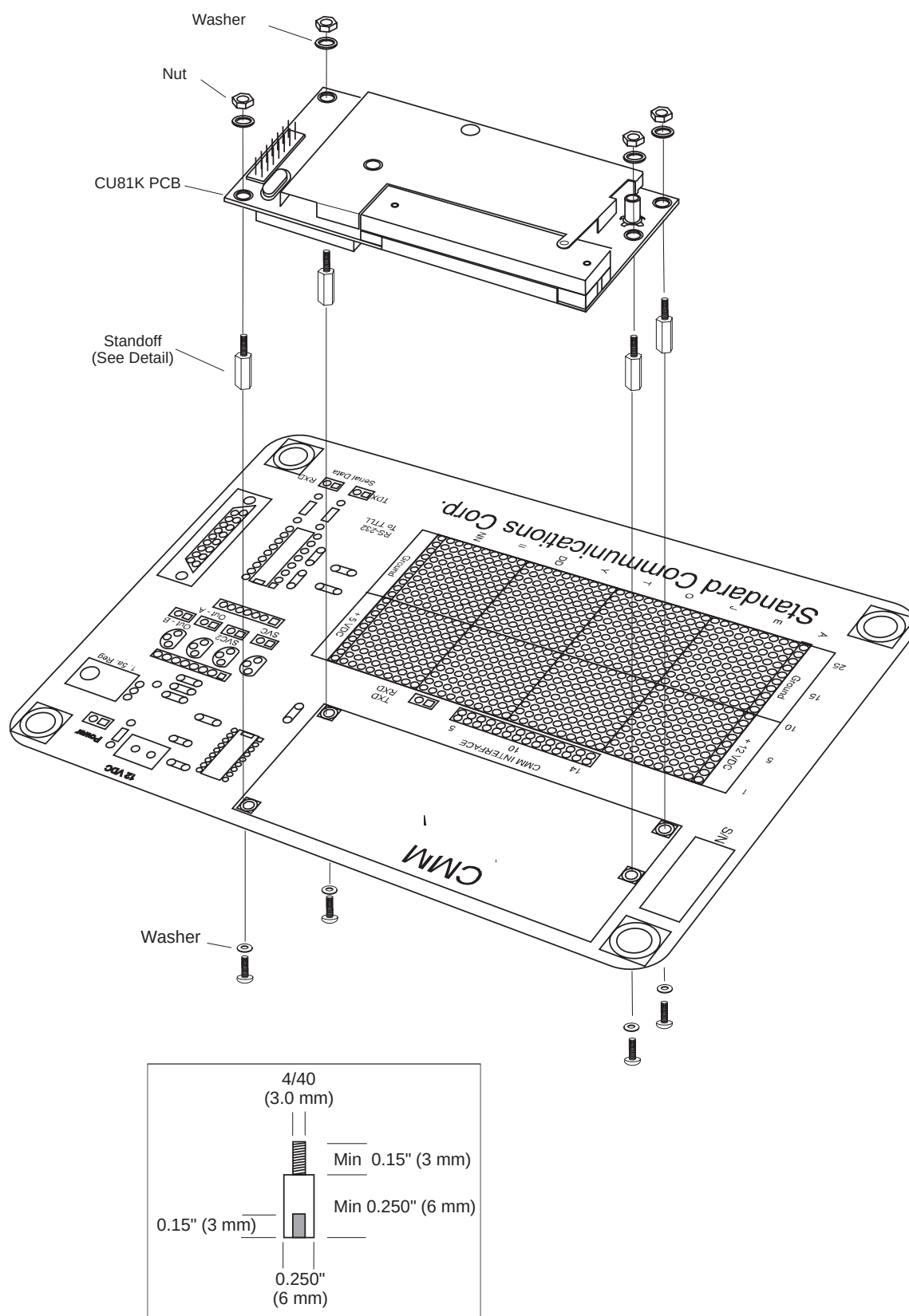
Figure 1. Mounting Details
