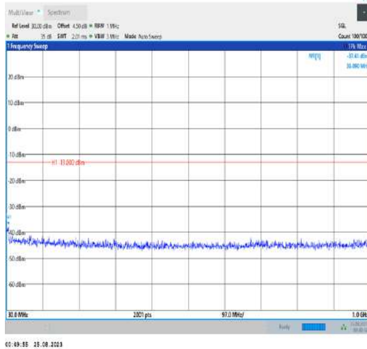
Band42_20MHz_QPSK_43190_1RB#0_30~1000_30~100 0
