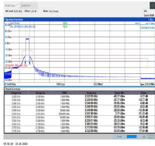
Band42_5MHz_QPSK_43115_25RB#0
