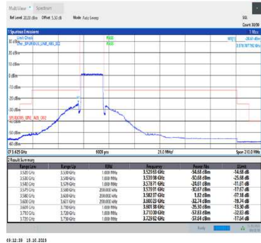
Band42_20MHz_QPSK_43490_100RB#0
