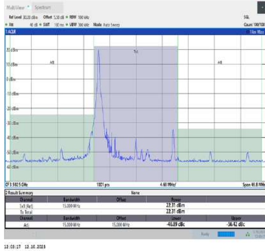
42(3550-3600)-15MHz-QPSK-43515-1RB#0-PASS
