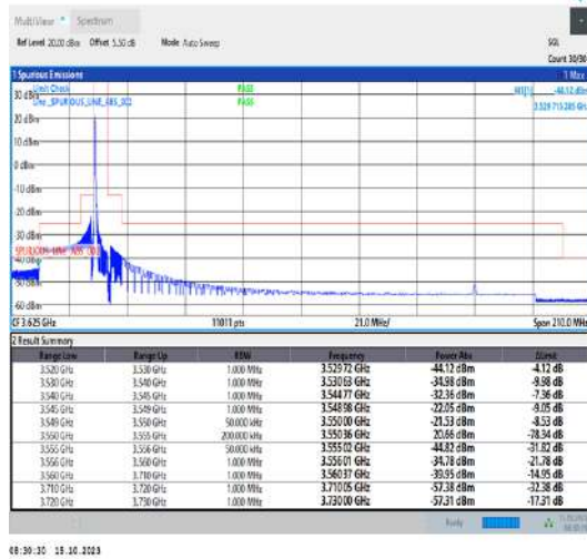
Band42_5MHz_QPSK_43115_1RB#0
