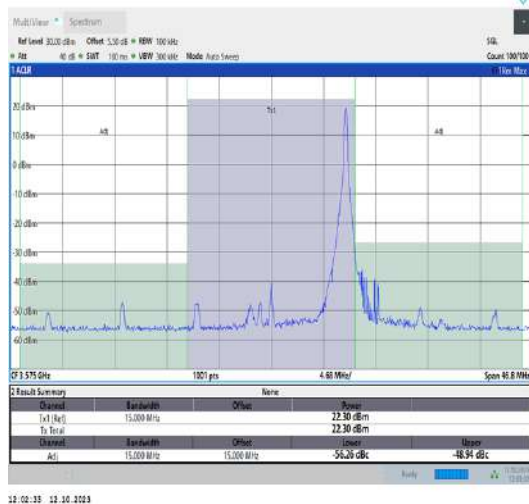
42(3550-3600)-15MHz-QPSK-43340-1RB#74-PASS
