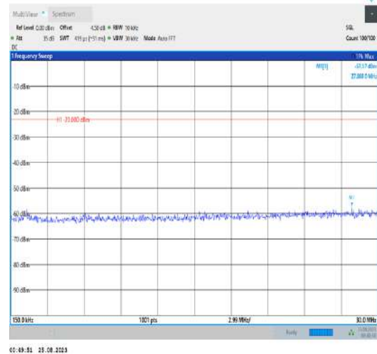
Band42_20MHz_QPSK_43190_1RB#0_0.15~30_0.15~ 30
