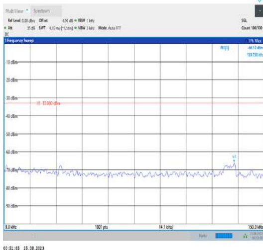
Band42_20MHz_QPSK_43490_1RB#0_0.009~0.15_0.009~0.15
