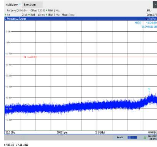
Band42_20MHz_QPSK_43340_1RB#0_20000~40000_20000~40000
