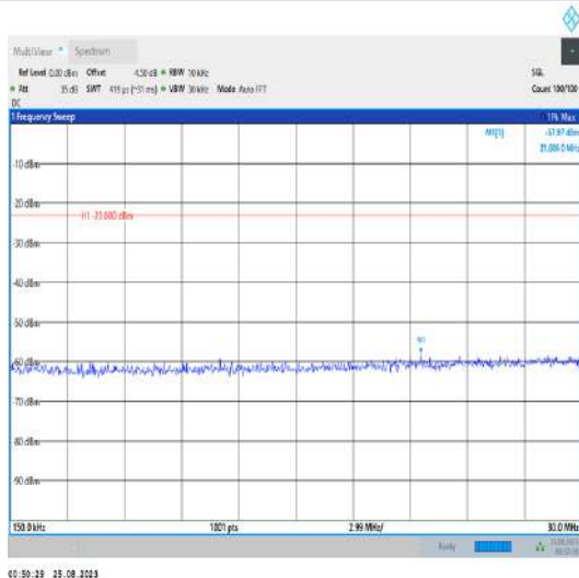
Band42_20MHz_QPSK_43340_1RB#0_0.15~30_0.15~30
