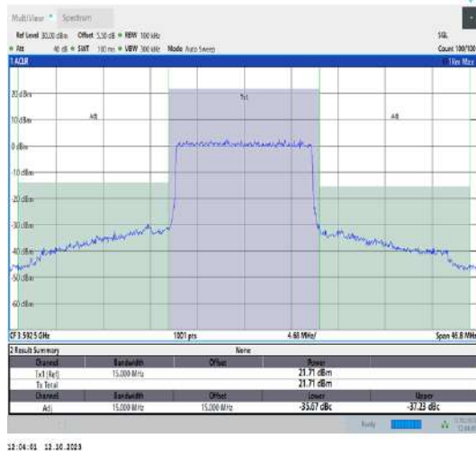
42(3550-3600)-15MHz-QPSK-43515-75RB#0-PASS
