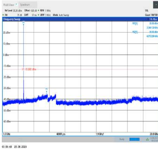
Band42_20MHz_QPSK_43340_1RB#0_1000~20000_1000~20000
