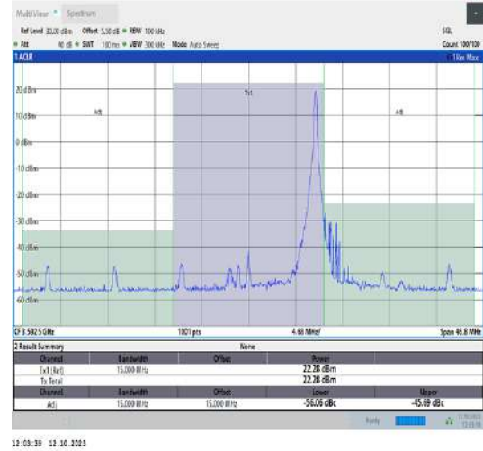
42(3550-3600)-15MHz-QPSK-43515-1RB#74-PASS
