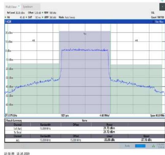
42(3550-3600)-15MHz-QPSK-43340-75RB#0-PASS
