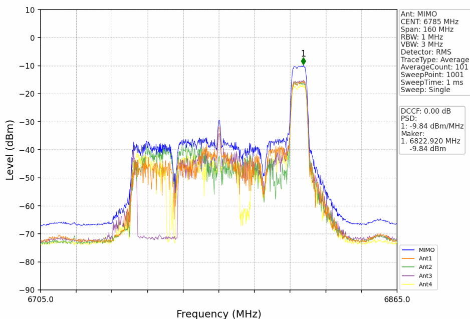
802.11ax(HEW80)_HCH_6785MHz_RU52+26_Right_MIMO_NTNV
