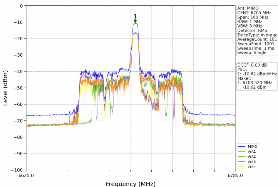
802.11ax(HEW80)_MCH_6705MHz_RU52_Mid_MIMO_NTNV
