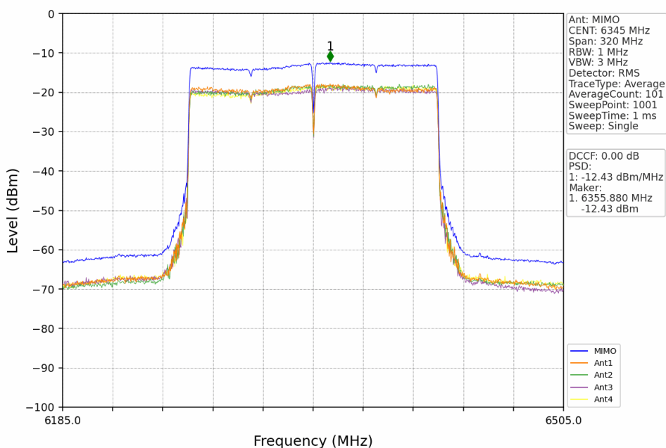
802.11ax(HEW160)_HCH_6345MHz_2xRU996_Left_MIMO_NTNV
