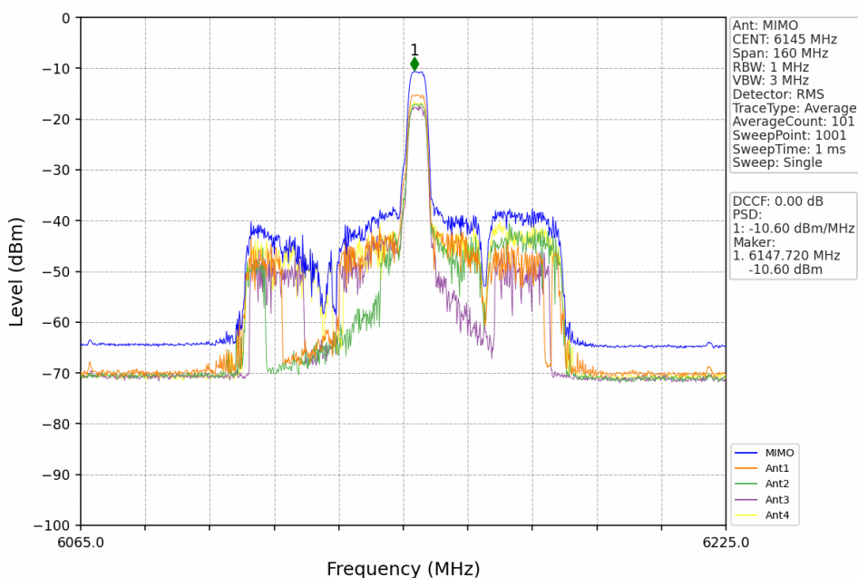
802.11ax(HEW80)_MCH_6145MHz_RU52_Mid_MIMO_NTNV
