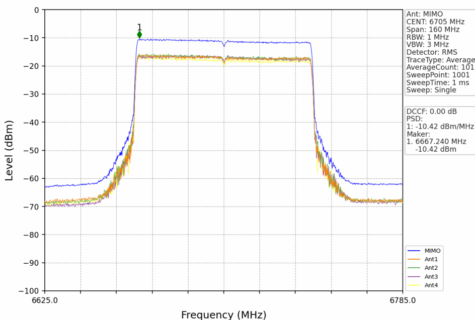
802.11ax(HEW80)_MCH_6705MHz_RU996_Left_MIMO_NTNV
