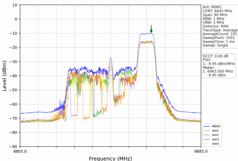
802.11ax(HEW40)_HCH_6845MHz_RU484_Left_MIMO_NTNV
