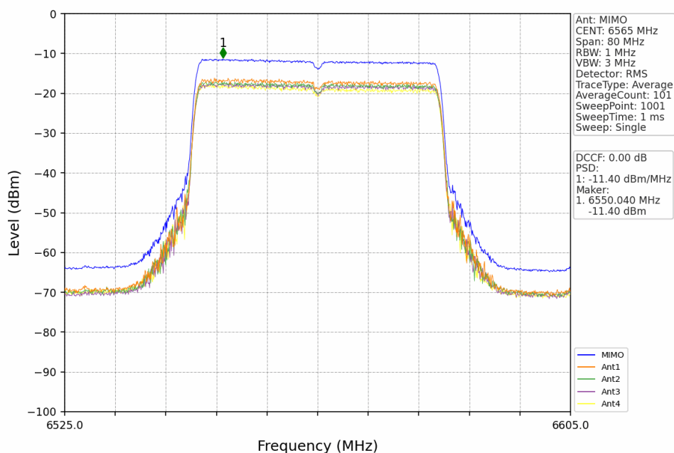
802.11ax(HEW40)_LCH_6565MHz_RU484_Left_MIMO_NTNV
