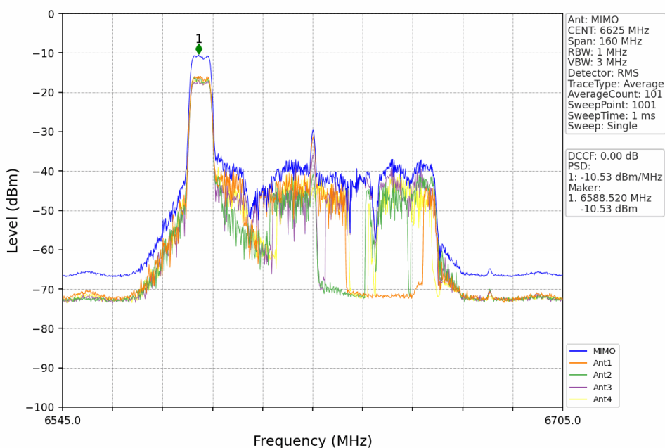
802.11ax(HEW80)_LCH_6625MHz_RU52+26_Left_MIMO_NTNV
