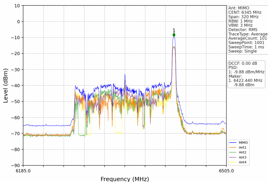
802.11ax(HEW160)_HCH_6345MHz_RU52_Right_MIMO_NTNV
