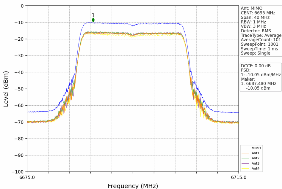
802.11ax(HEW20)_MCH_6695MHz_RU242_Left_MIMO_NTNV
