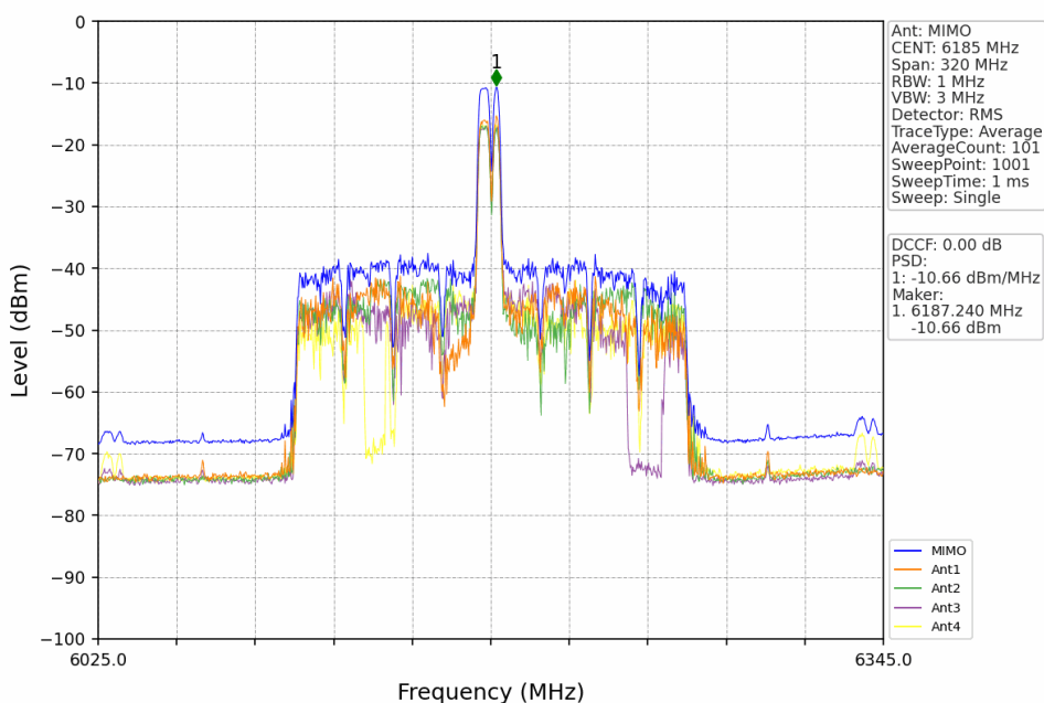
802.11ax(HEW160)_MCH_6185MHz_RU52+26_Mid_MIMO_NTNV
