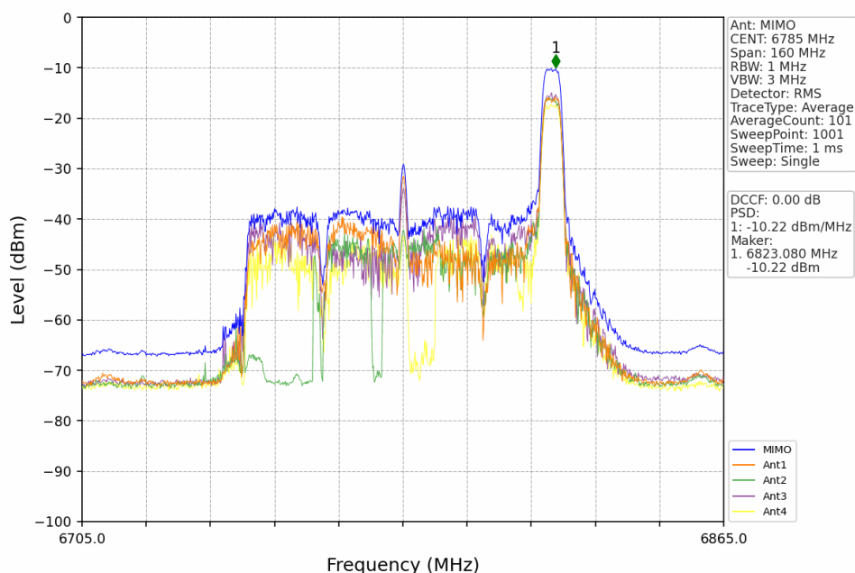
802.11ax(HEW80)_HCH_6785MHz_RU52+26_Right_MIMO_NTNV
