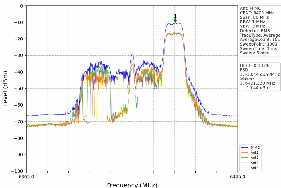
802.11ax(HEW40)_HCH_6405MHz_RU484_Left_MIMO_NTNV
