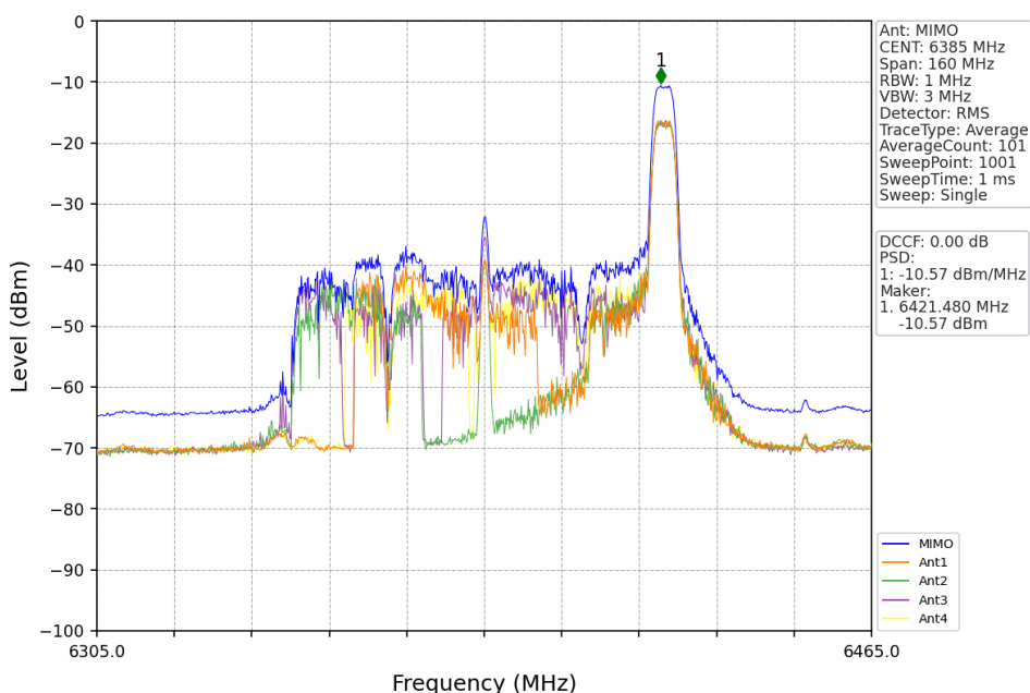
802.11ax(HEW80)_HCH_6385MHz_RU52+26_Right_MIMO_NTNV
