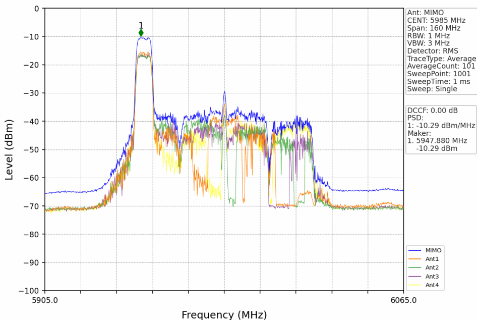
802.11ax(HEW80)_LCH_5985MHz_RU52+26_Left_MIMO_NTNV
