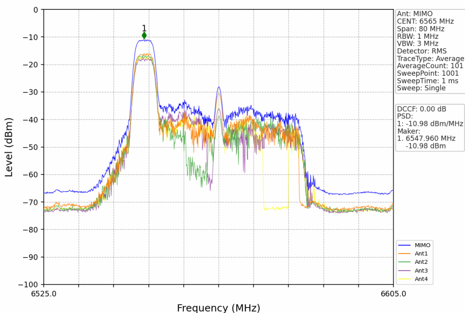
802.11ax(HEW40)_LCH_6565MHz_RU52_Left_MIMO_NTNV
