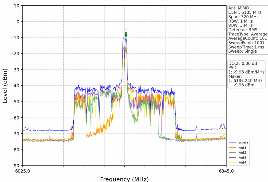
802.11ax(HEW160)_MCH_6185MHz_RU52+26_Mid_MIMO_NTNV
