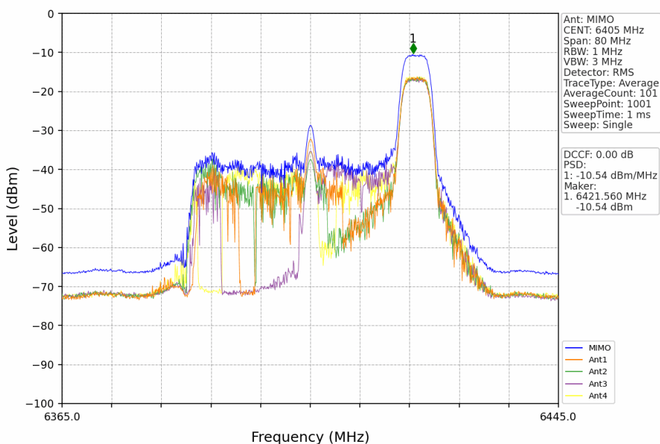
802.11ax(HEW40)_HCH_6405MHz_RU52_Right_MIMO_NTNV
