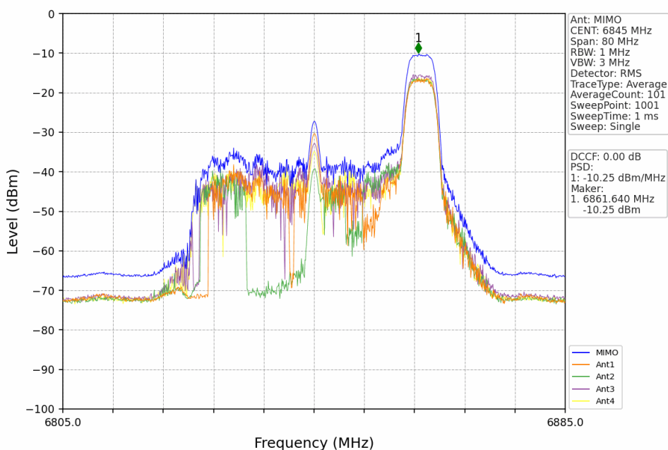
802.11ax(HEW40)_HCH_6845MHz_RU52_Right_MIMO_NTNV
