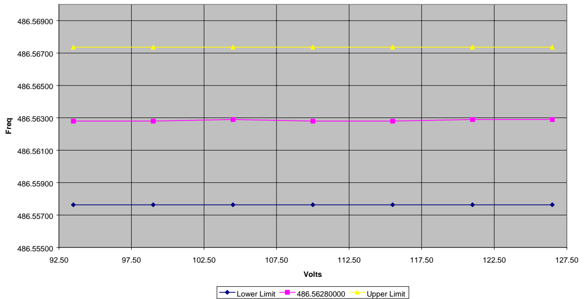
Uplink - 60-055902 - 486.5625MHz Frequency Stability - Voltage
