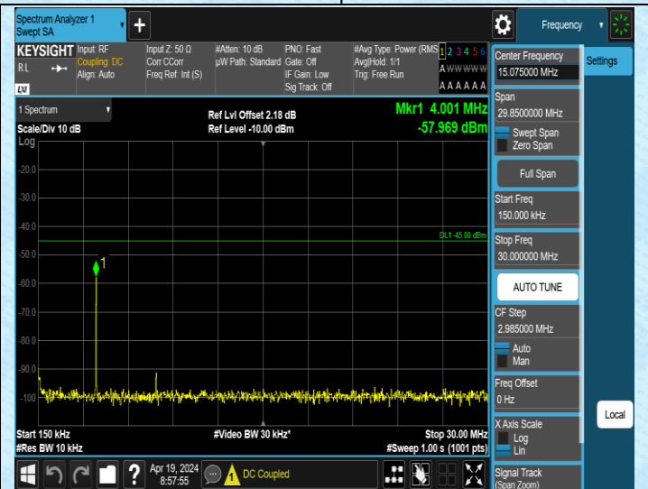
Band41_5MHz_QPSK_40590_1RB#0_0.15~30_0.15~30
