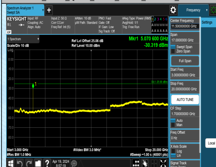
Band41_5MHz_QPSK_40065_1RB#0_3000~20000_3000~2000
