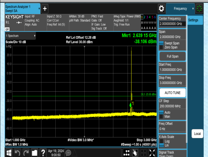
Band41_5MHz_QPSK_41215_1RB#0_1000~3000_1000~3000
