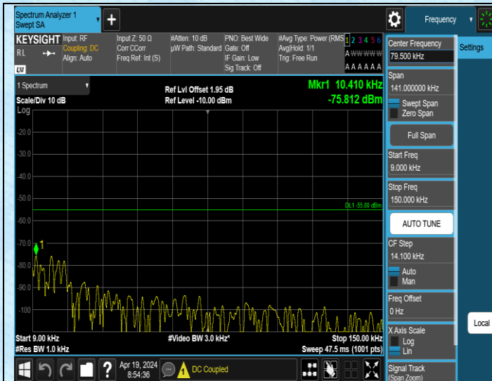
Band41_5MHz_QPSK_40065_1RB#0_0.009~0.15_0.009~0.15
