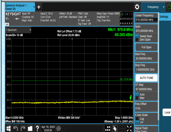
Band41_5MHz_QPSK_40065_1RB#0_30~1000_30~1000
