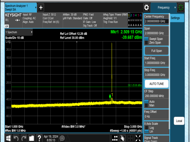
Band41_5MHz_QPSK_40065_1RB#0_1000~3000_1000~3000
