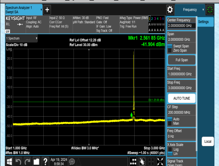
Band41_5MHz_QPSK_40590_1RB#0_1000~3000_1000~3000
