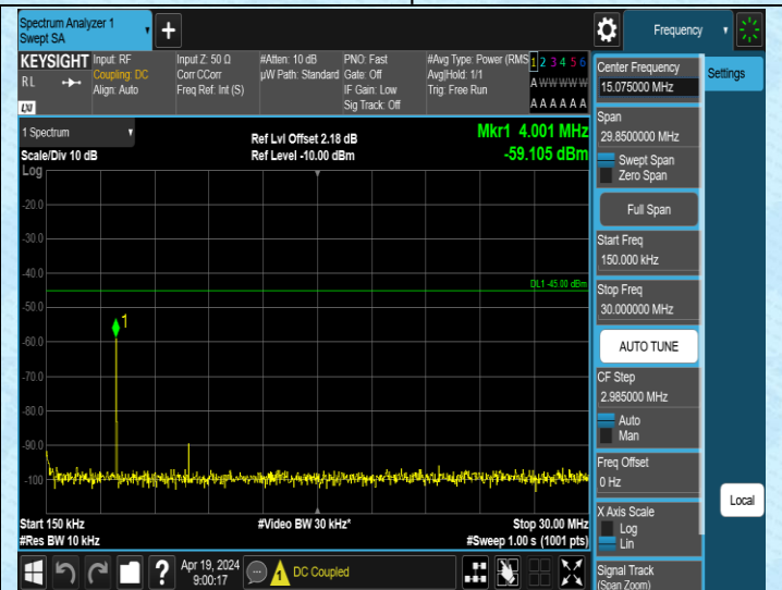
Band41_5MHz_QPSK_41215_1RB#0_0.15~30_0.15~30
