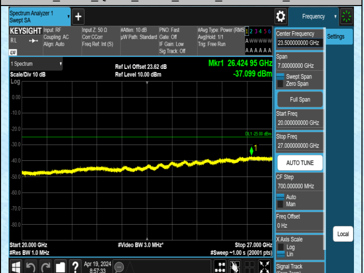
Band41_5MHz_QPSK_40065_1RB#0_20000~27000_20000~27
