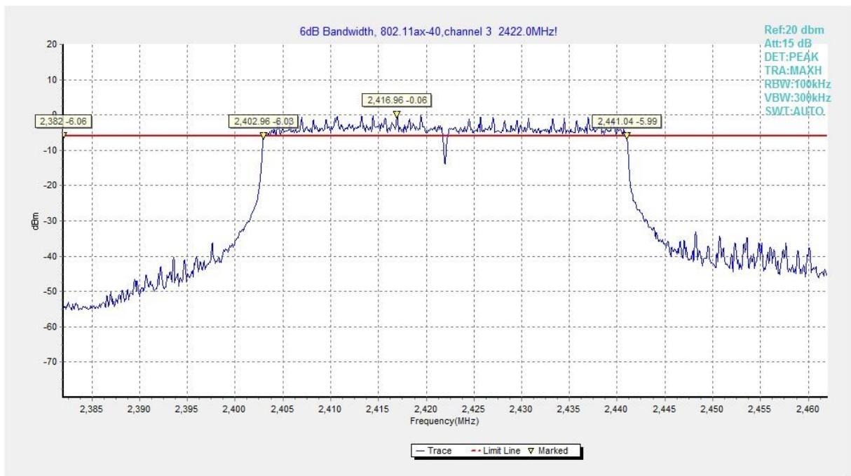
Fig.A.4.16 Occupied 6dB Bandwidth (802.11ax-HE40, Ch 3)
