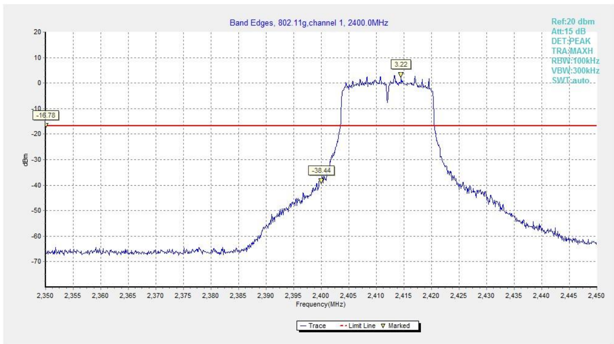
Fig.A.5.15 Band Edges (802.11g, Ch 1)
