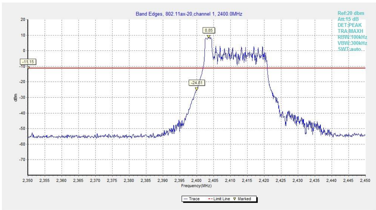
Fig.A.5.17 Band Edges (802.11ax-HE20 RU26-index0, Ch 1)
