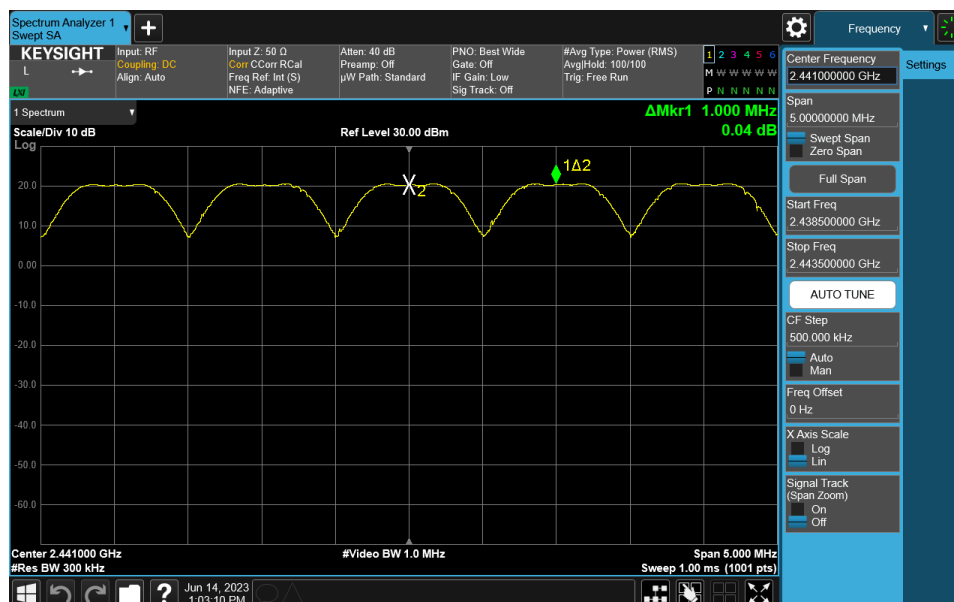
Plot 7-15. Channel Spacing Plot (Bluetooth, GFSK, ePA)
