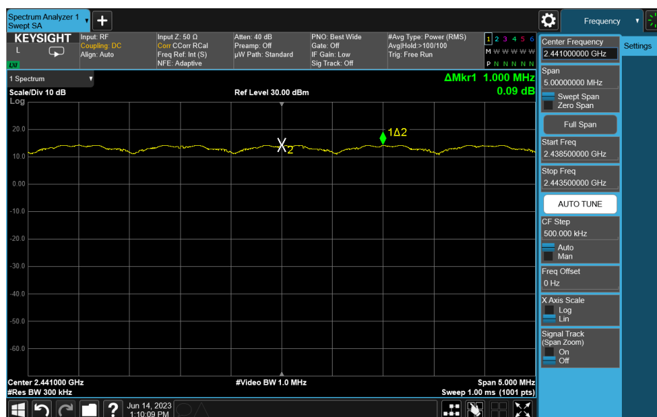
Plot 7-16. Channel Spacing Plot (Bluetooth, 8DPSK, ePA)
