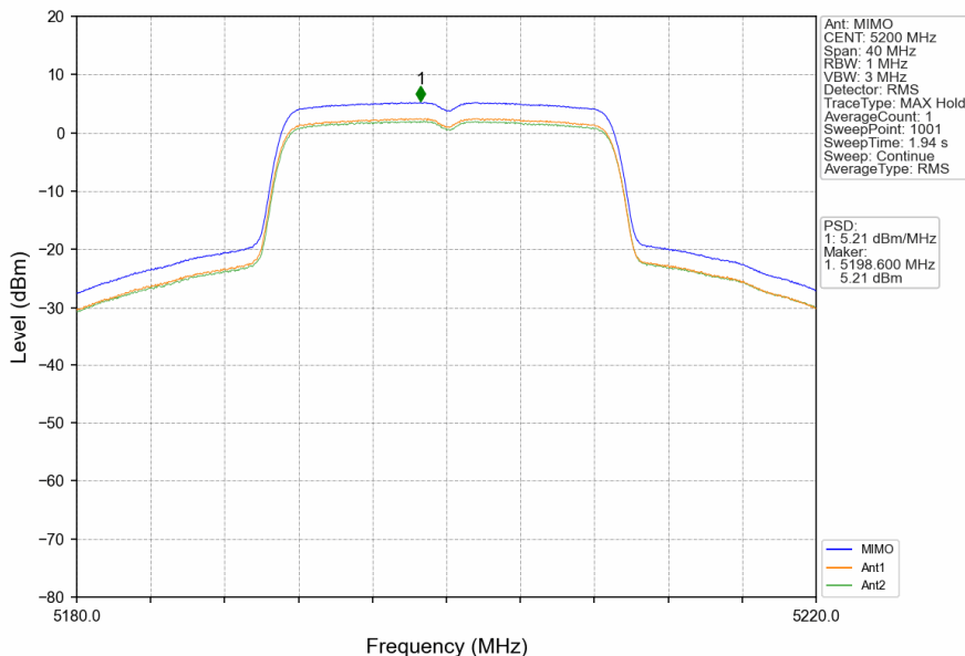
802.11ac(VHT20)_MCH_5200MHz_MIMO_NTNV
