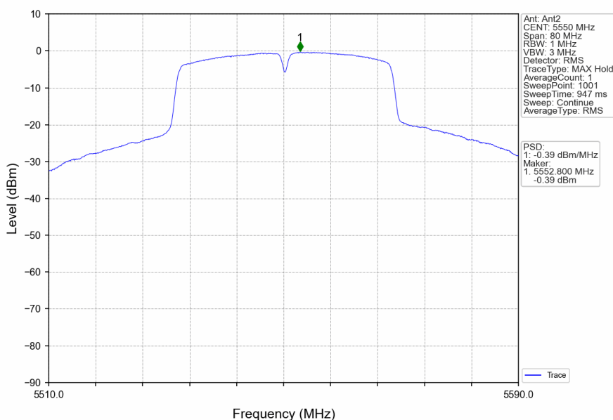
802.11n(HT40)_MCH_5550MHz_Ant2_NTNV
