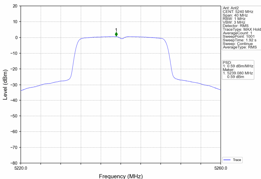
802.11n(HT20)_HCH_5240MHz_Ant2_NTNV
