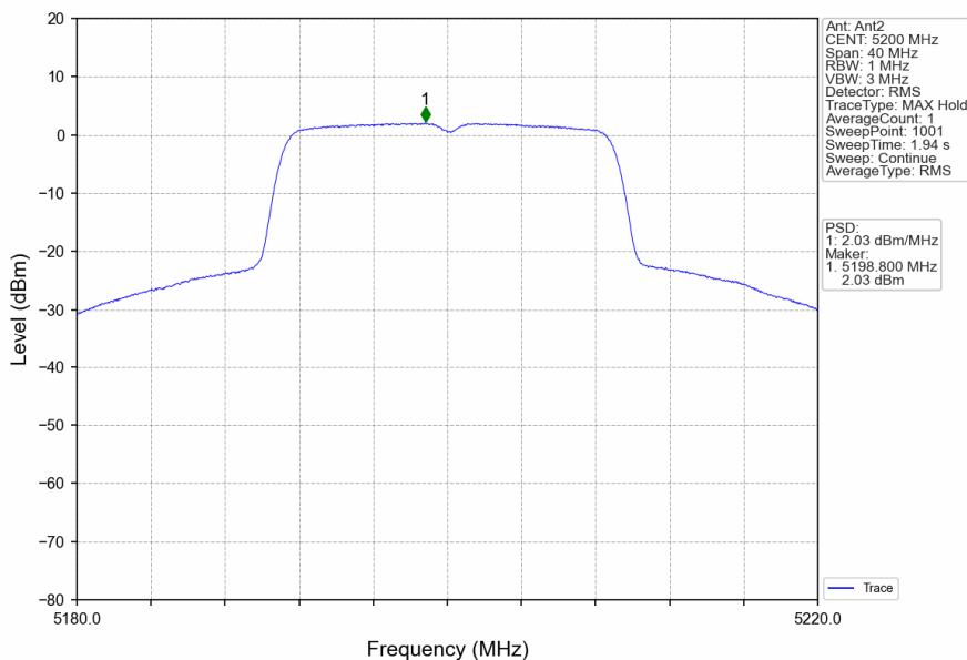
802.11ac(VHT20)_MCH_5200MHz_MIMO_NTNV
