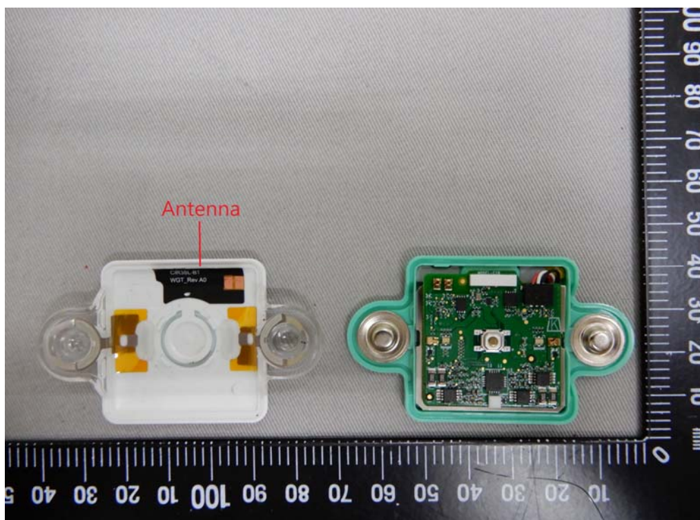
Antenna (Model No: Q-ecg-wu5)
