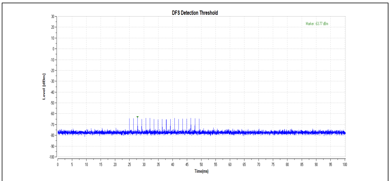
802.11ac (VHT80) _5530_Reference
