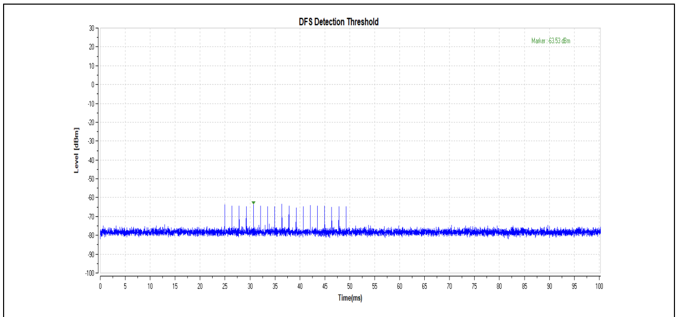
802.11ac (VHT80) _5290_Reference
