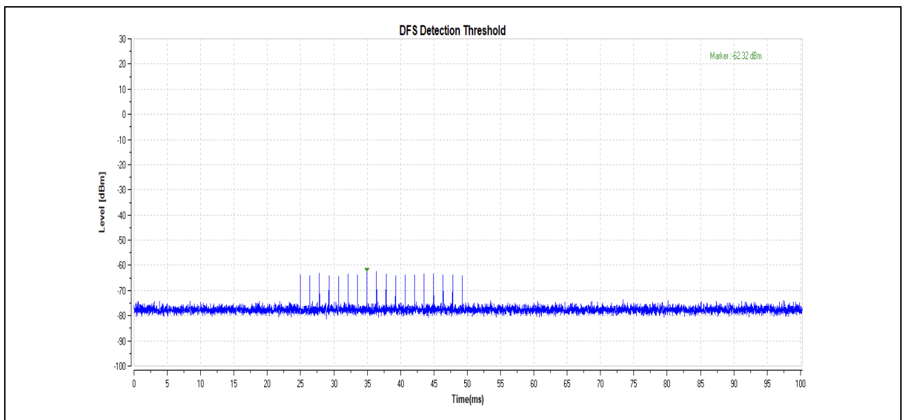
802.11a_5500_Reference
