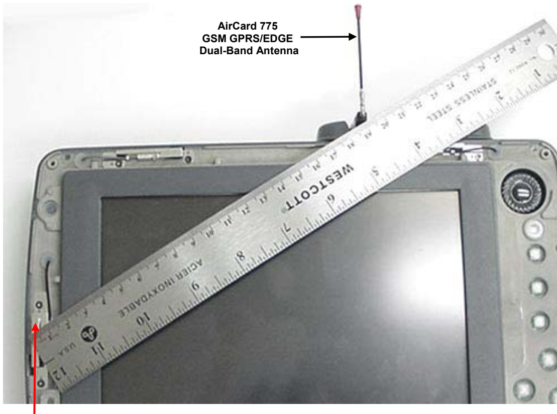
Bluetooth Antenna
