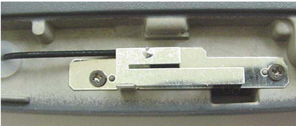
Internal Bluetooth PIFA Antenna
