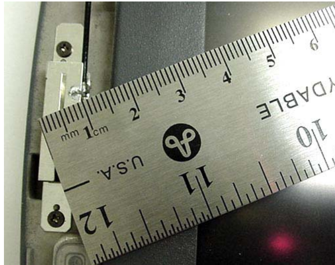
Internal Bluetooth PIFA Antenna
