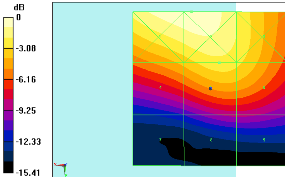
Fig B.4 HAC RF E-Field LTE Band41 PC3 16QAM CH41490
