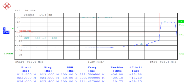
1.4MHz_Low_QPSK_6@0
