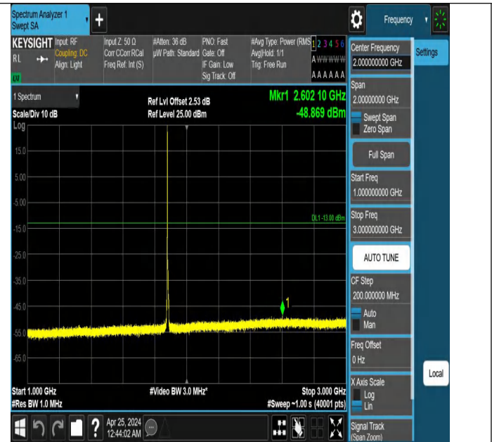
Band2_5MHz_QPSK_18900_1RB#0_1000~3000_1000~3000
