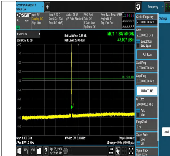
Band2_3MHz_QPSK_18900_1RB#14_1000~3000_1000~3000
