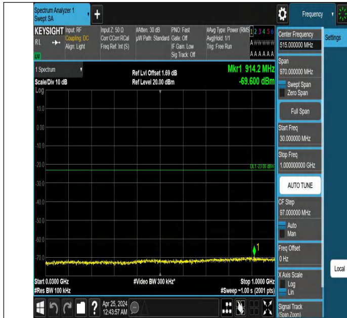
Band2_5MHz_QPSK_18900_1RB#0_30~1000_30~1000
