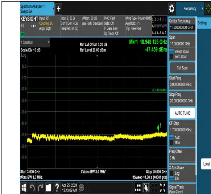
Band2_5MHz_QPSK_18625_1RB#0_3000~20000_3000~20000
