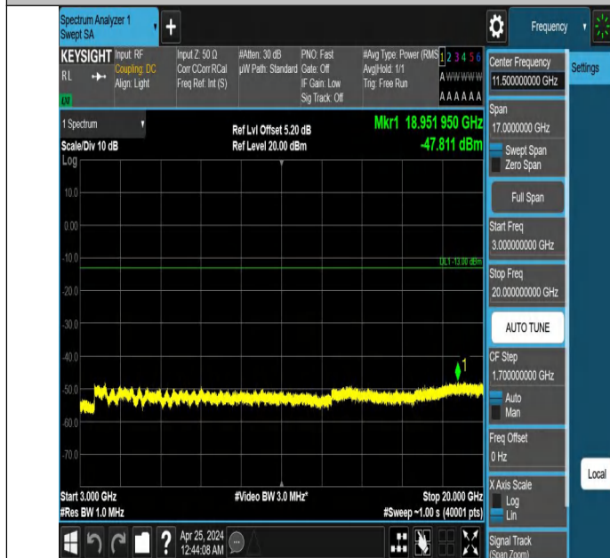
Band2_5MHz_QPSK_18900_1RB#0_3000~20000_3000~20000
