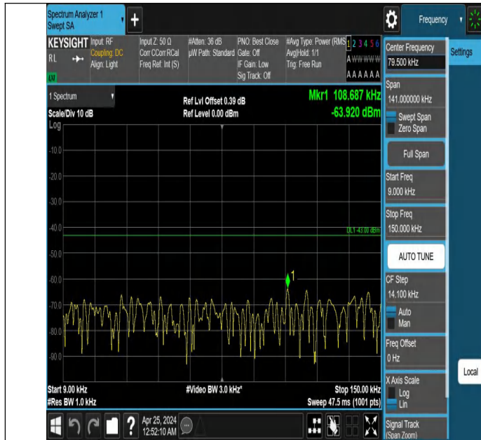
Band2_10MHz_QPSK_18900_1RB#0_0.009~0.15_0.009~0.15
