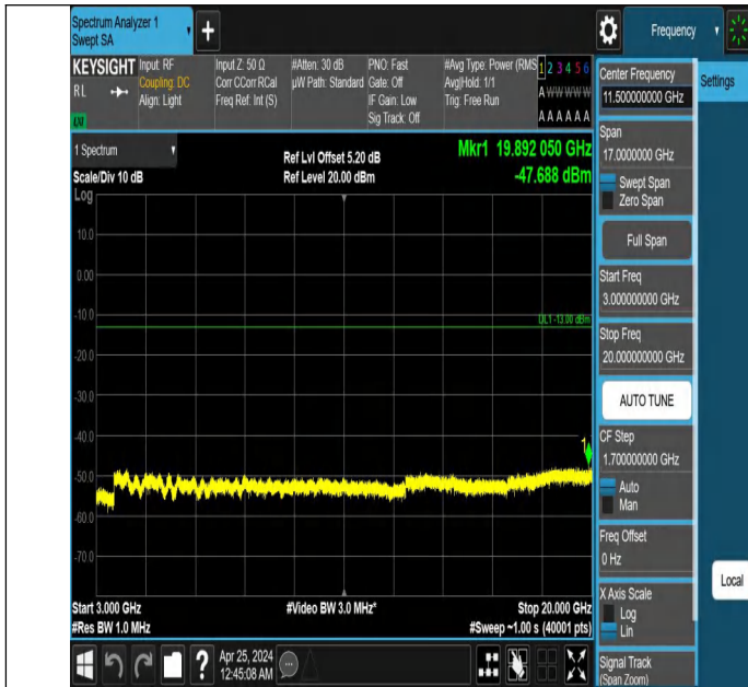
Band2_5MHz_QPSK_19175_1RB#0_3000~20000_3000~20000
