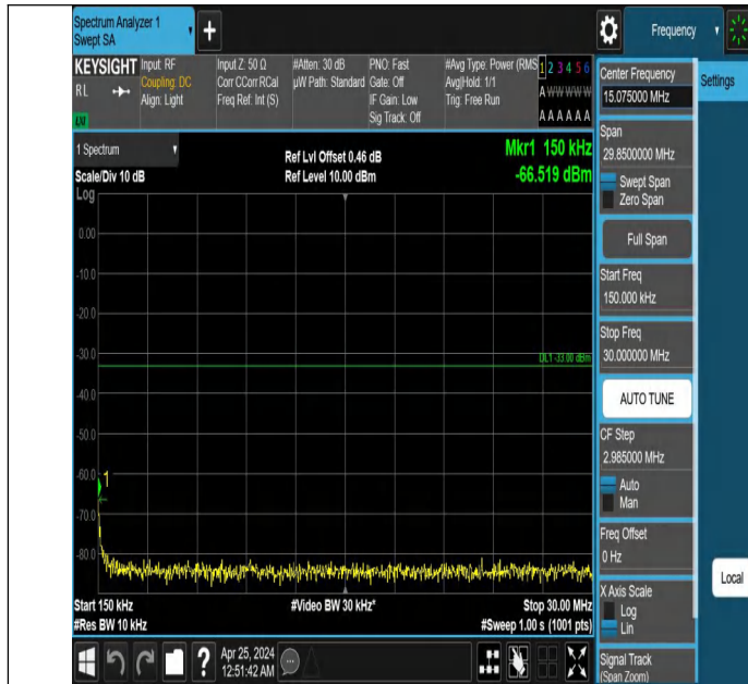
Band2_10MHz_QPSK_18650_1RB#49_0.15~30_0.15~30
