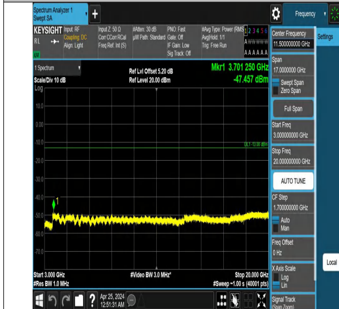
Band2_10MHz_QPSK_18650_1RB#0_3000~20000_3000~20000
