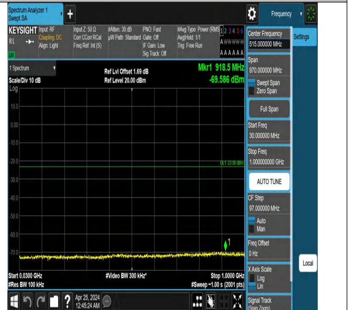
Band2_5MHz_QPSK_19175_1RB#24_30~1000_30~1000
