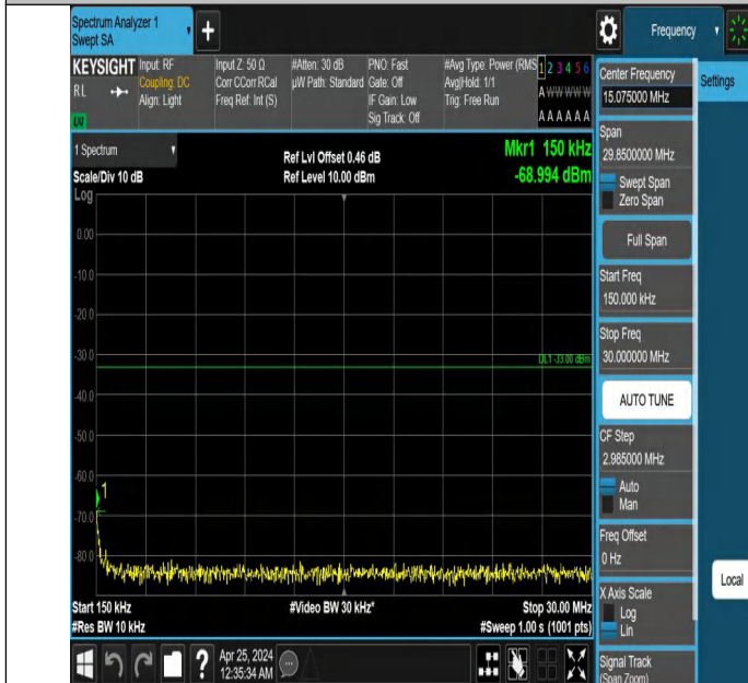
Band2_3MHz_QPSK_18900_1RB#14_0.15~30_0.15~30
