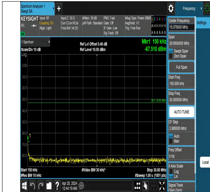
Band2_5MHz_QPSK_18900_1RB#24_0.15~30_0.15~30
