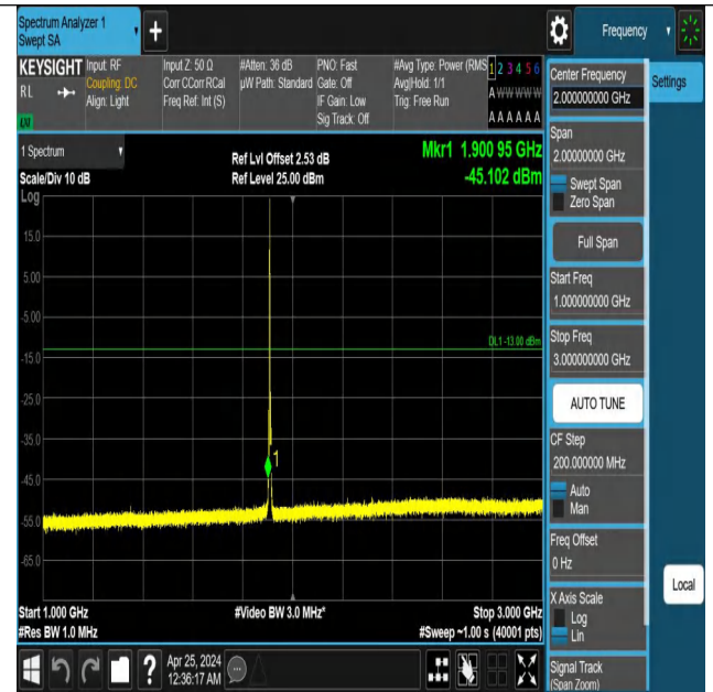
Band2_3MHz_QPSK_19185_1RB#0_1000~3000_1000~3000
