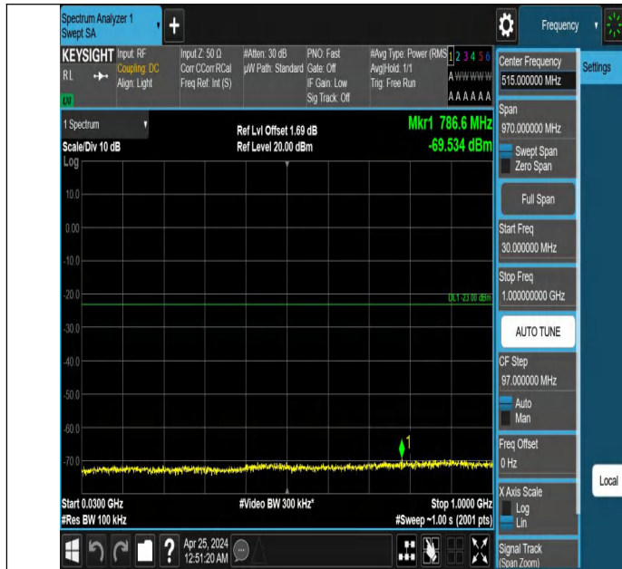
Band2_10MHz_QPSK_18650_1RB#0_30~1000_30~1000
