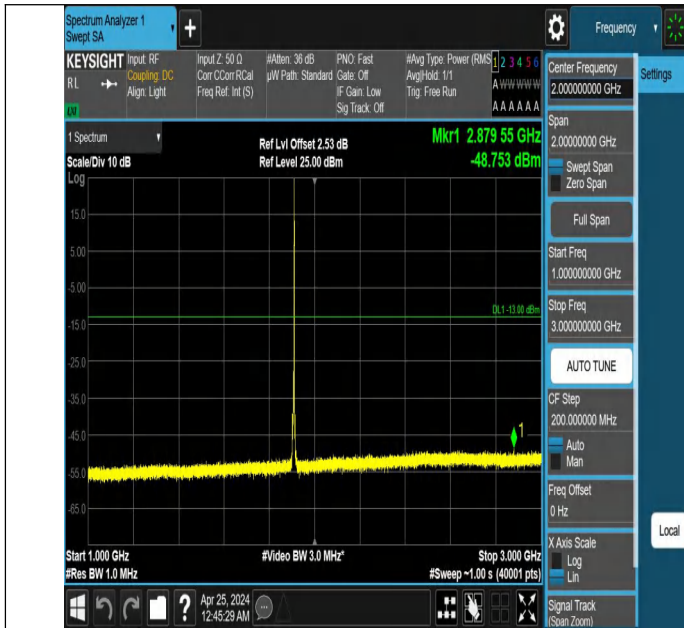
Band2_5MHz_QPSK_19175_1RB#24_1000~3000_1000~3000
