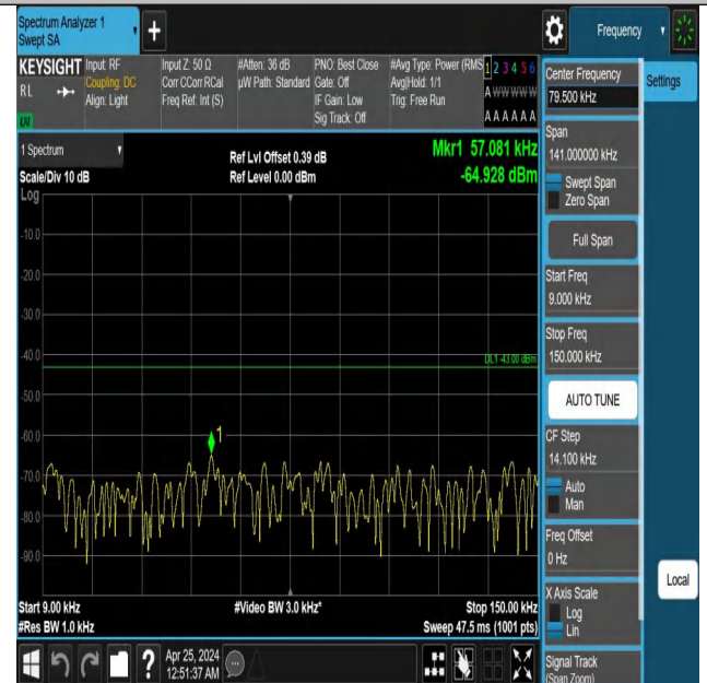
Band2_10MHz_QPSK_18650_1RB#49_0.009~0.15_0.009~0.15
