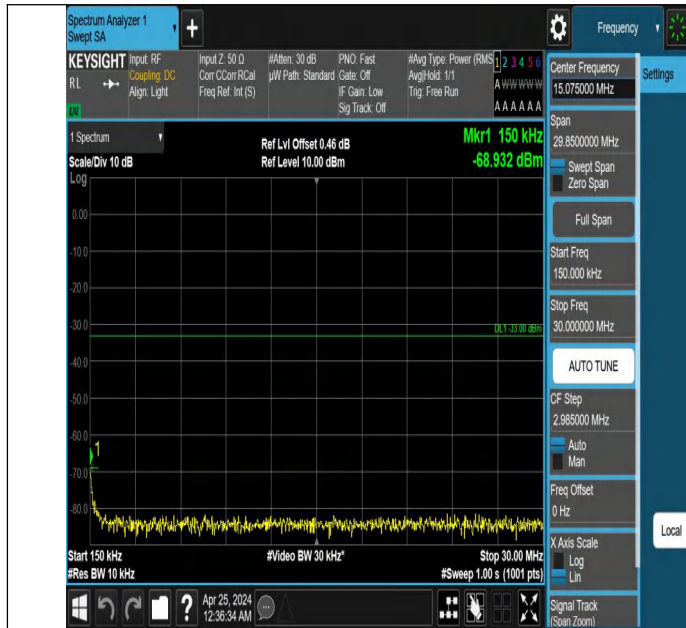
Band2_3MHz_QPSK_19185_1RB#14_0.15~30_0.15~30
