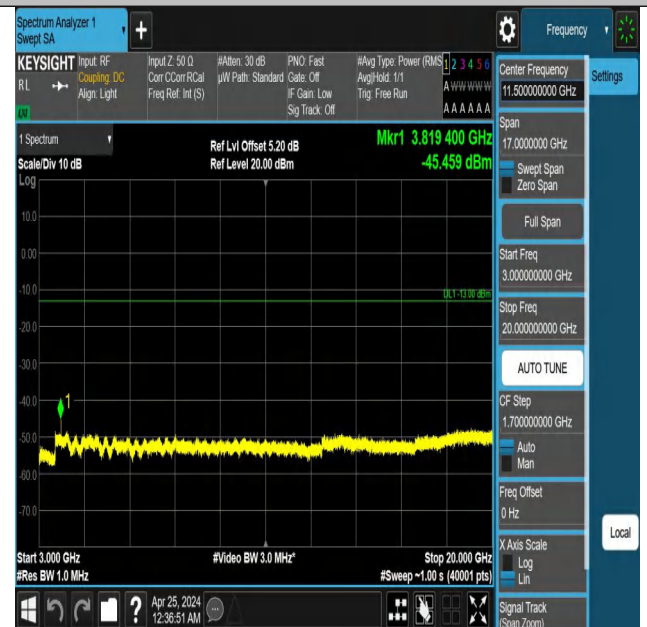
Band2_3MHz_QPSK_19185_1RB#14_3000~20000_3000~20000
