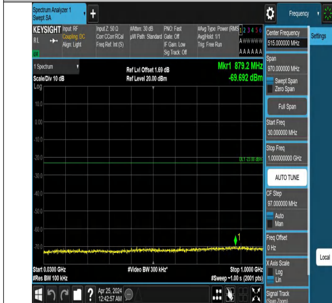
Band2_5MHz_QPSK_18625_1RB#0_30~1000_30~1000
