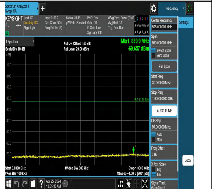
Band2_3MHz_QPSK_18900_1RB#14_30~1000_30~1000
