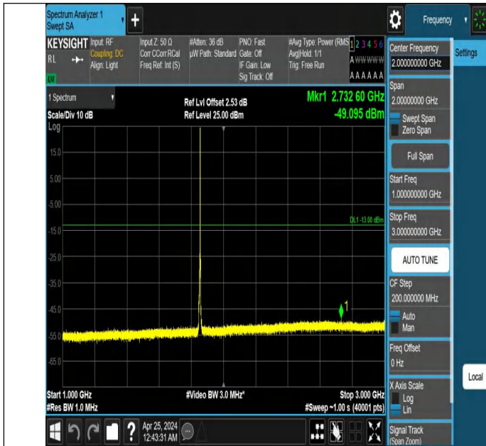
Band2_5MHz_QPSK_18625_1RB#24_1000~3000_1000~3000
