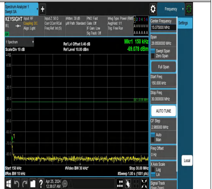
Band2_3MHz_QPSK_19185_1RB#0_0.15~30_0.15~30
