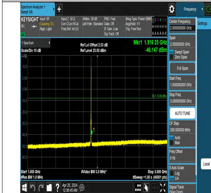
Band2_3MHz_QPSK_19185_1RB#14_1000~3000_1000~3000
