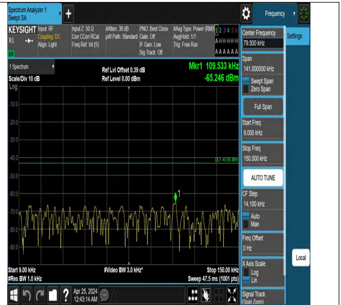
Band2_5MHz_QPSK_18625_1RB#24_0.009~0.15_0.009~0.15
