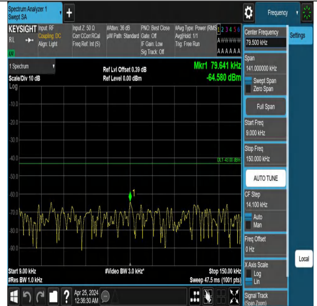
Band2_3MHz_QPSK_19185_1RB#14_0.009~0.15_0.009~0.15
