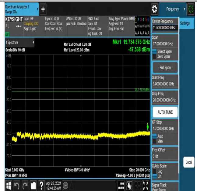
Band2_5MHz_QPSK_18900_1RB#24_3000~20000_3000~20000
