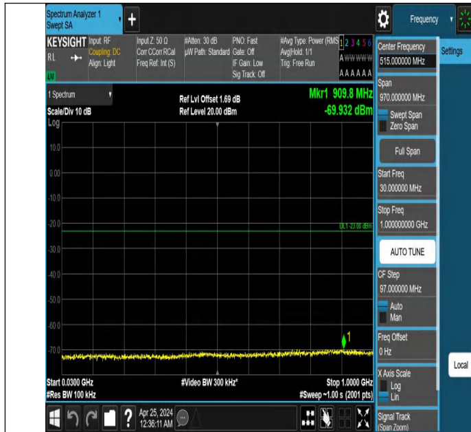
Band2_3MHz_QPSK_19185_1RB#0_30~1000_30~1000
