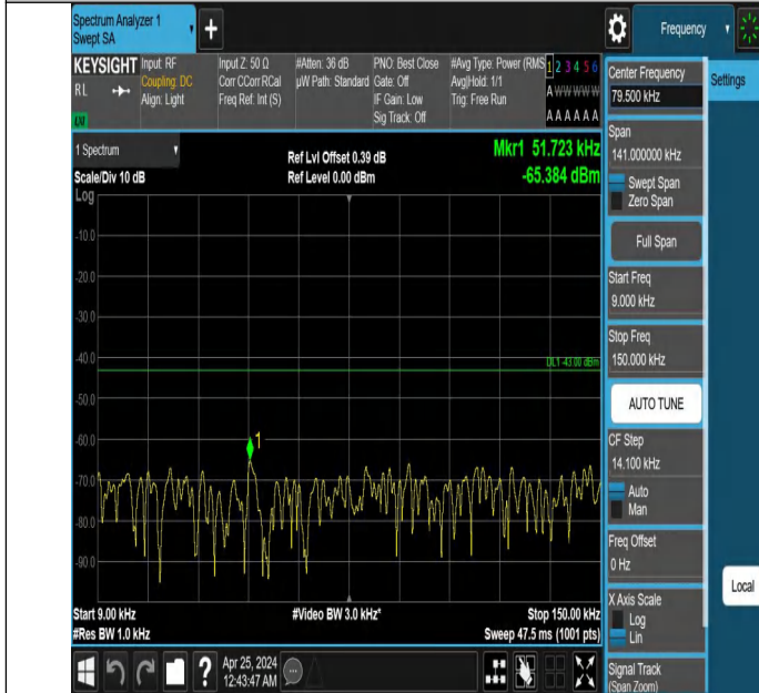
Band2_5MHz_QPSK_18900_1RB#0_0.009~0.15_0.009~0.15
