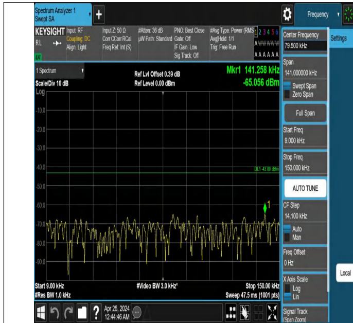
Band2_5MHz_QPSK_19175_1RB#0_0.009~0.15_0.009~0.15
