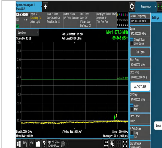
Band2_5MHz_QPSK_19175_1RB#0_30~1000_30~1000
