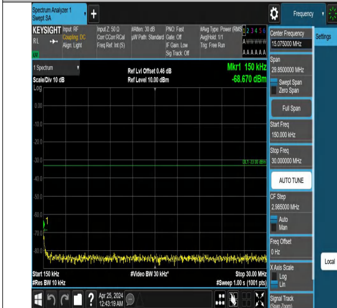
Band2_5MHz_QPSK_18625_1RB#24_0.15~30_0.15~30
