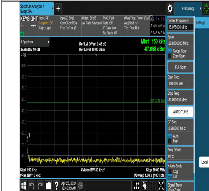
Band2_5MHz_QPSK_19175_1RB#24_0.15~30_0.15~30
