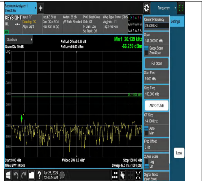
Band2_5MHz_QPSK_19175_1RB#24_0.009~0.15_0.009~0.15
