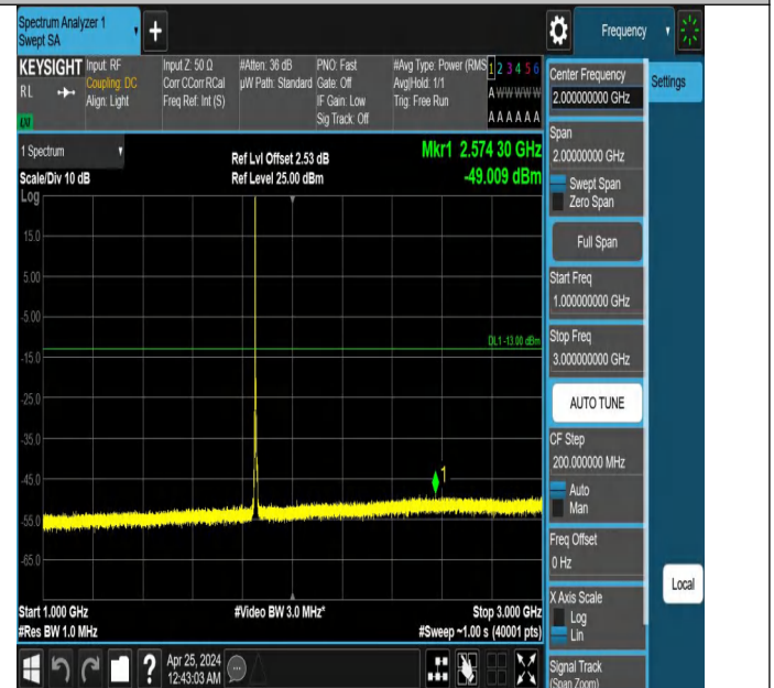
Band2_5MHz_QPSK_18625_1RB#0_1000~3000_1000~3000
