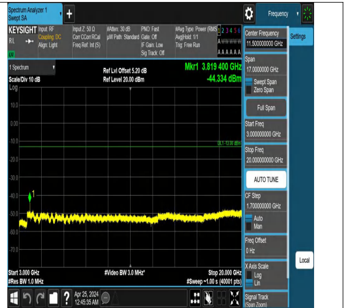
Band2_5MHz_QPSK_19175_1RB#24_3000~20000_3000~20000
