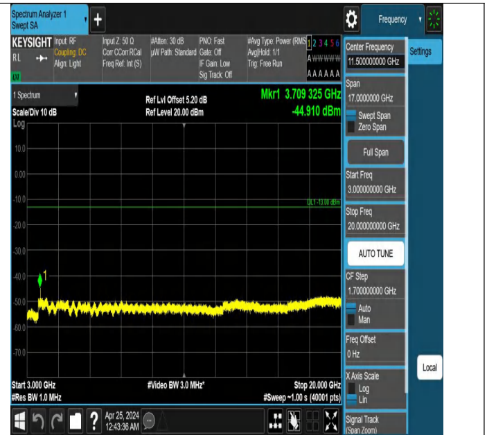
Band2_5MHz_QPSK_18625_1RB#24_3000~20000_3000~20000
