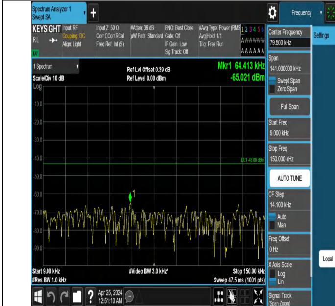
Band2_10MHz_QPSK_18650_1RB#0_0.009~0.15_0.009~0.15
