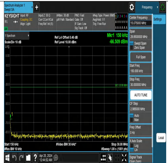
Band2_5MHz_QPSK_19175_1RB#0_0.15~30_0.15~30
