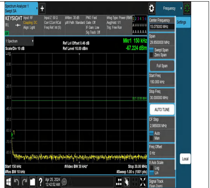
Band2_5MHz_QPSK_18625_1RB#0_0.15~30_0.15~30
