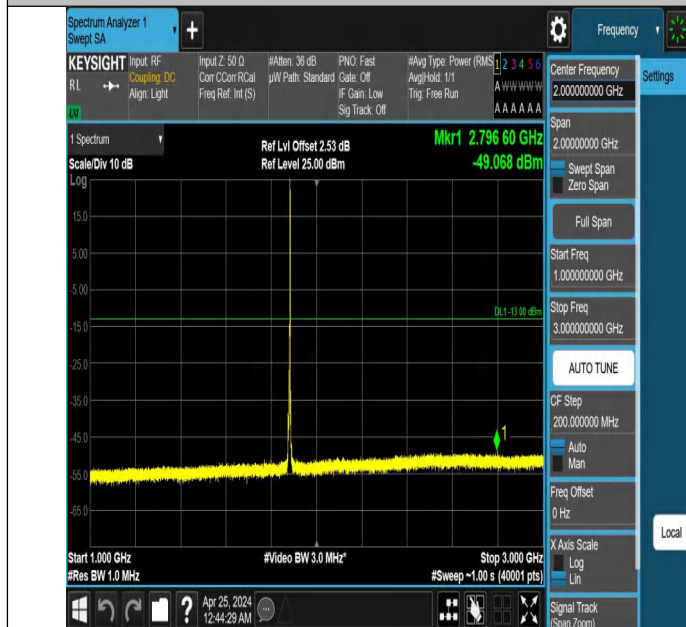
Band2_5MHz_QPSK_18900_1RB#24_1000~3000_1000~3000
