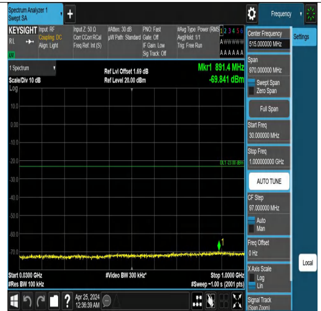
Band2_3MHz_QPSK_19185_1RB#14_30~1000_30~1000
