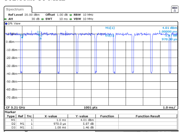
802.11ax-80 MHz
