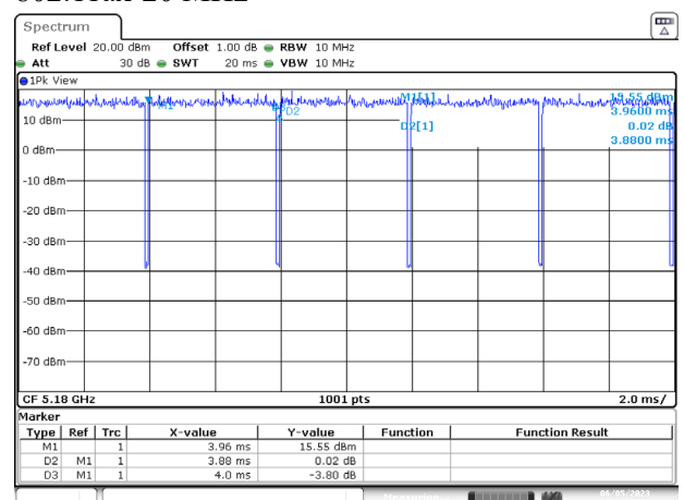
802.11ax-20 MHz
