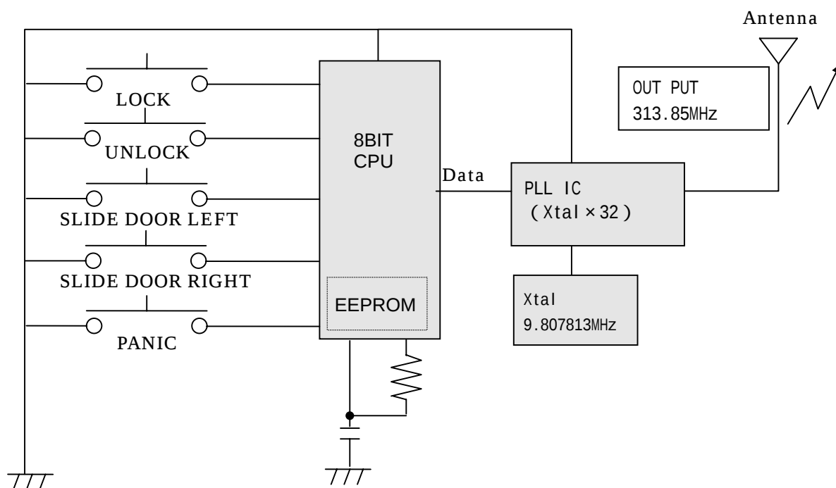
Figure 3.1 block diagram of the transmitter
