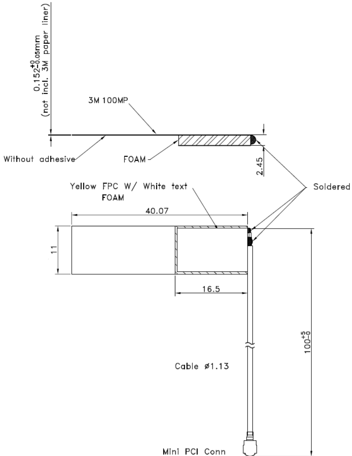
Figure 1 Physical Dimensions
