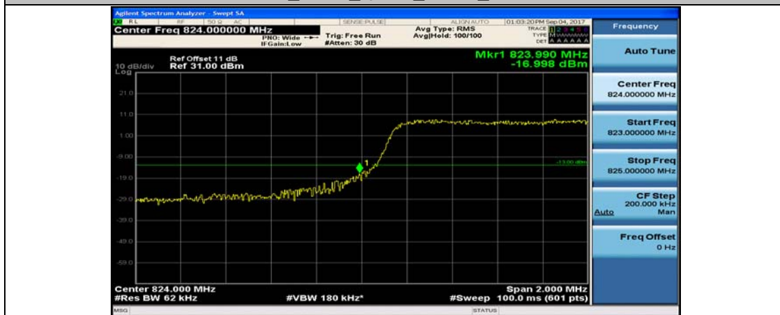
Band5_3MHz_16QAM_20415_15RB#0
