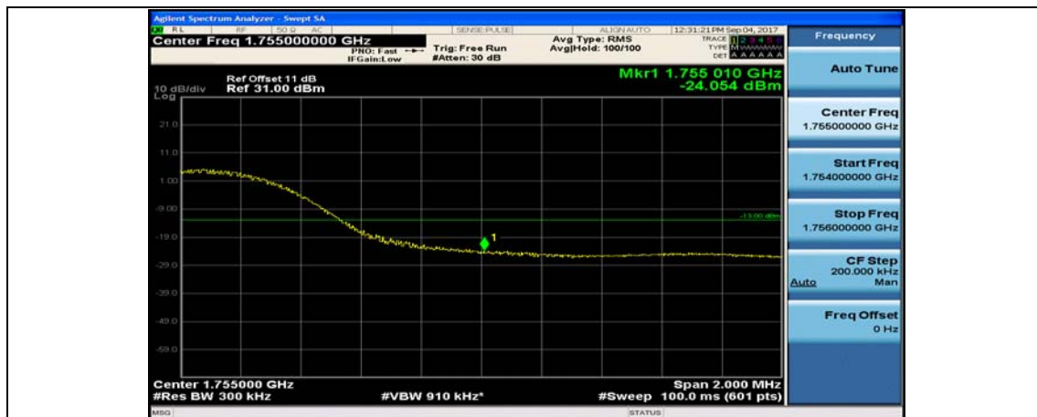
Band4_15MHz_16QAM_20325_75RB#0
