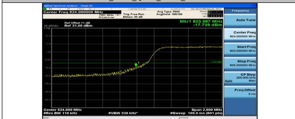
Band5_5MHz_16QAM_20425_25RB#0
