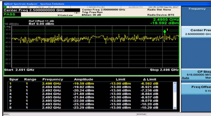
Band7_15MHz_16QAM_20825_75RB#0
