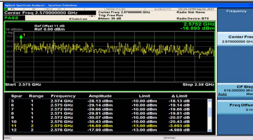
Band7_10MHz_16QAM_21400_50RB#0
