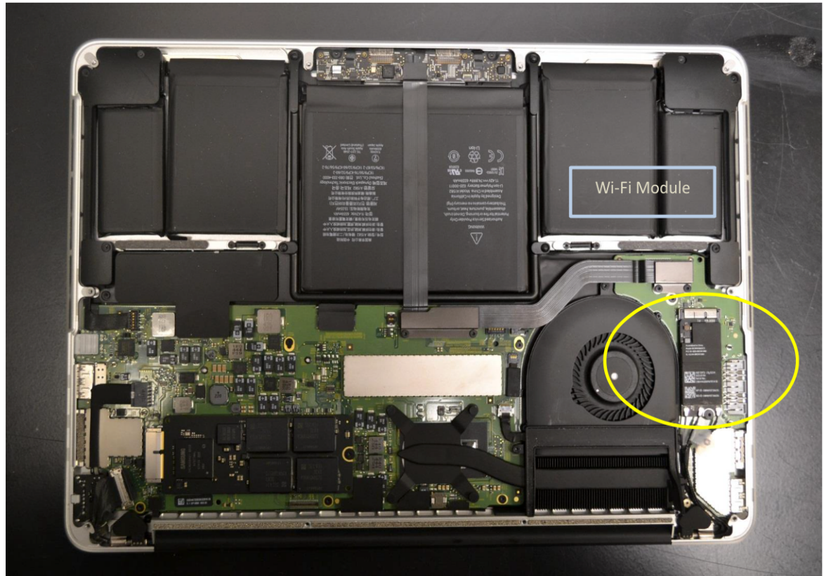
Wi-Fi Module location
