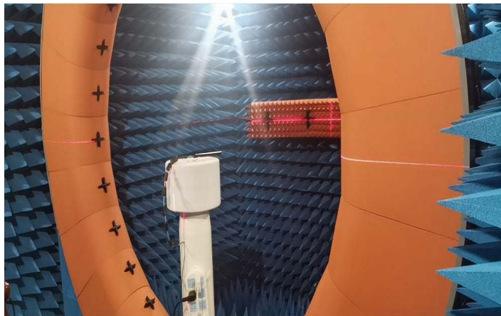
test instrument
