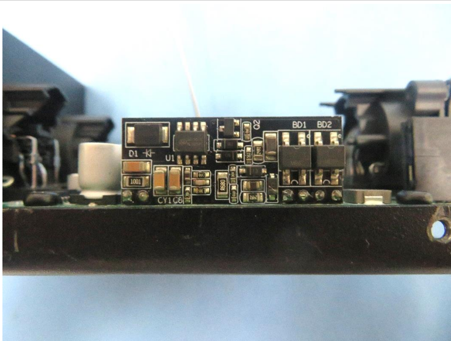
PCB View
