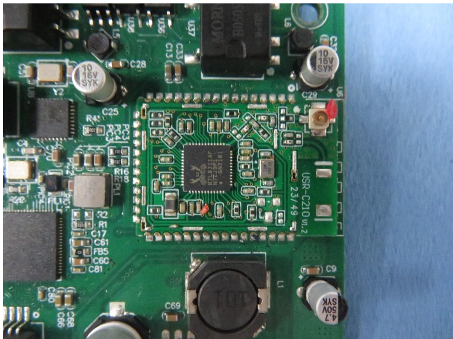
WIFI module PCB View
