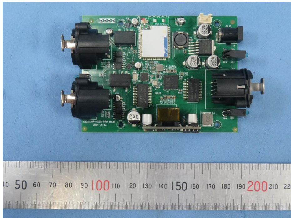
PCB View
