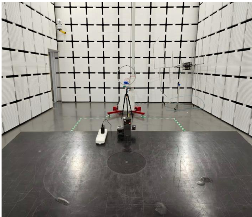
Spurious Radiation Emissions Test (<30M)
