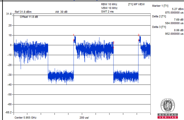
20MHz Preamble (RU26)
