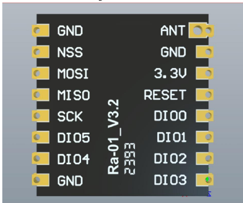
Ra-01 Figure 2.1 Ra-01Pin diagram
