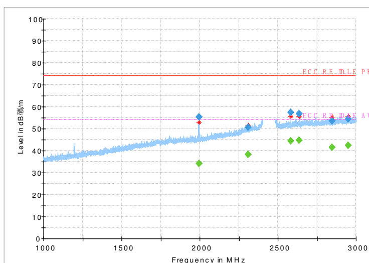
Fig.41 Radiated emission: GFSK, Ch78, 1GHz~3GHz
