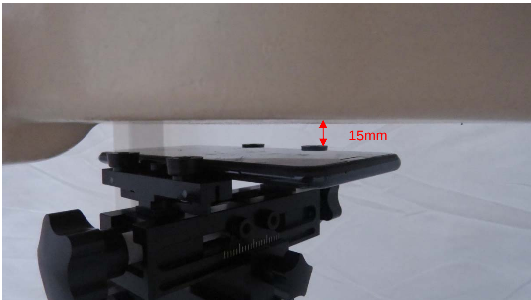
Picture 8: Front Side, the distance from handset to the bottom of the Phantom is 15mm
