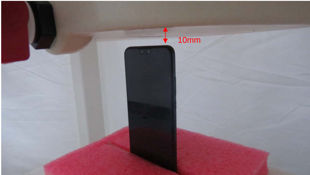
Picture 11: Top Edge, the distance from handset to the bottom of the Phantom is 10mm
