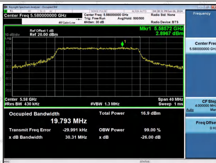
11AX20SISO-Ant1-5580
