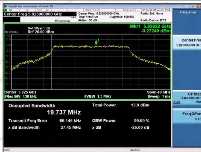
11AX20SISO-Ant1-5825
