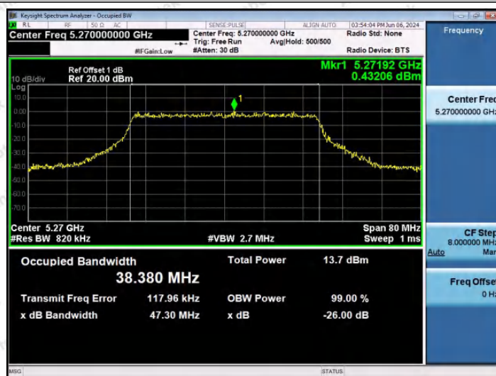
11AX40SISO-Ant1-5270
