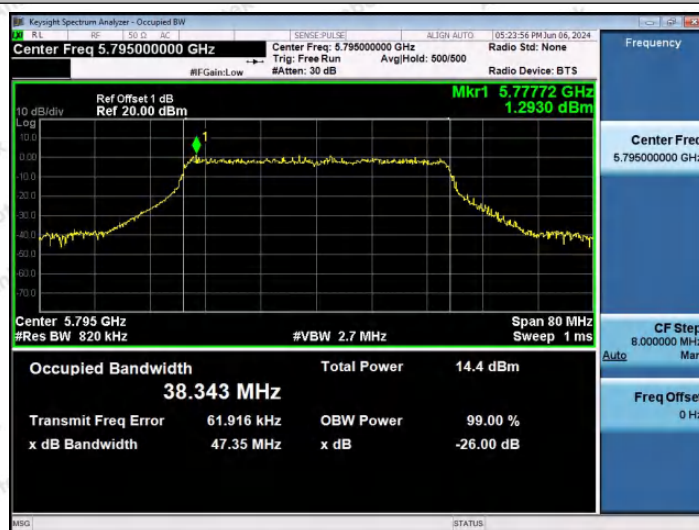
11AX40SISO-Ant1-5795
