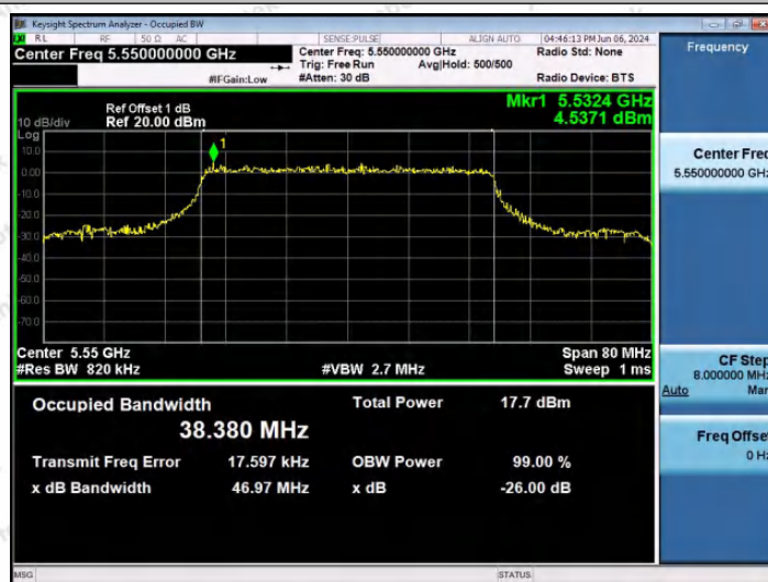
11AX40SISO-Ant1-5550
