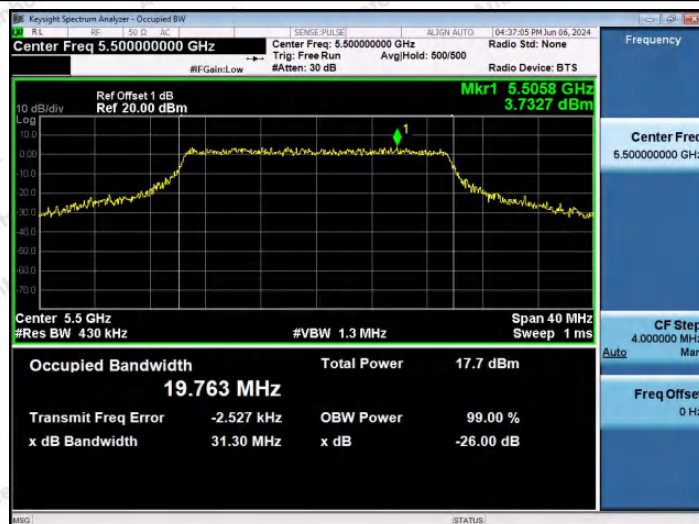
11AX20SISO-Ant1-5500
