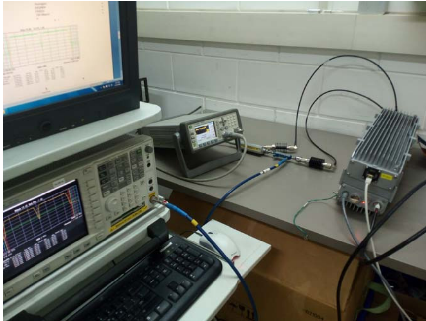
Photograph No.2 Occupied bandwidth emissions measurement setup
