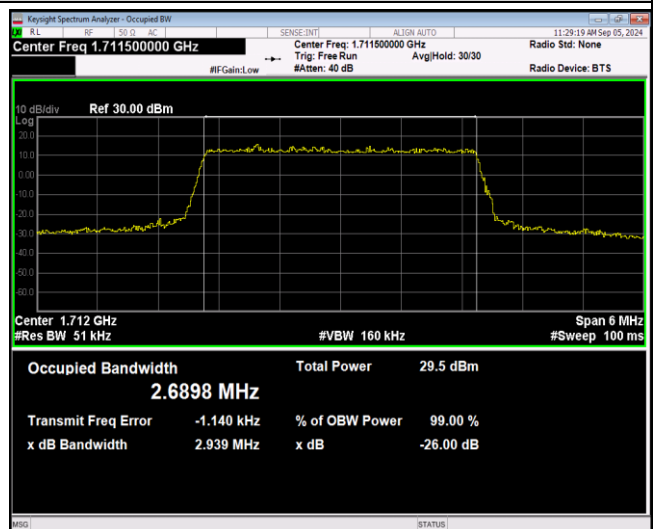
Band4-3MHz-16QAM-19965-15RB#0
