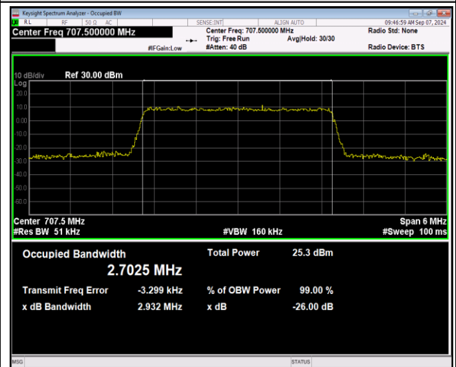
Band12-3MHz-16QAM-23025-15RB#0
