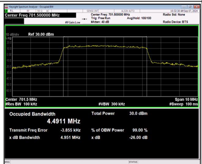
Band12-5MHz-16QAM-23035-25RB#0
