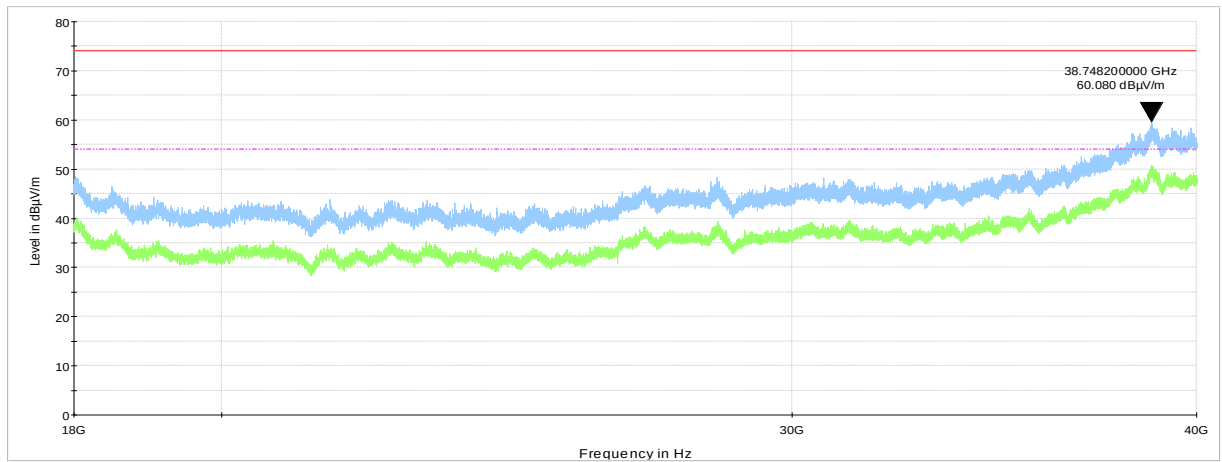
Plot 11.3.11 Radiated emission measurements from 18 to 40 GHz at the mid carrier frequency
