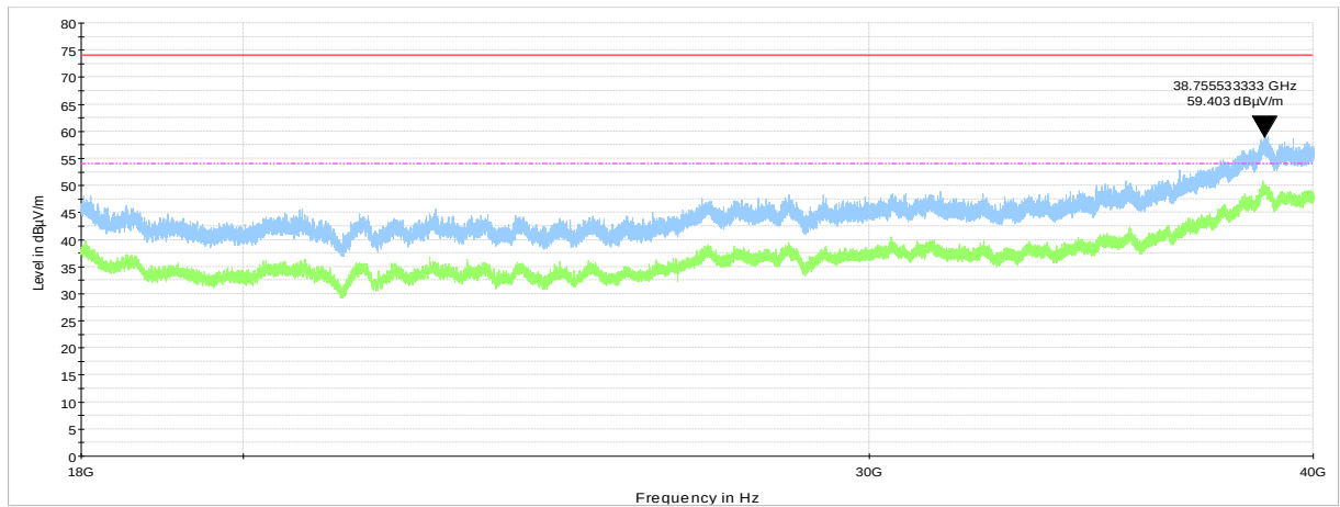
Plot 11.2.11 Radiated emission measurements from 18 to 40 GHz at the mid carrier frequency
