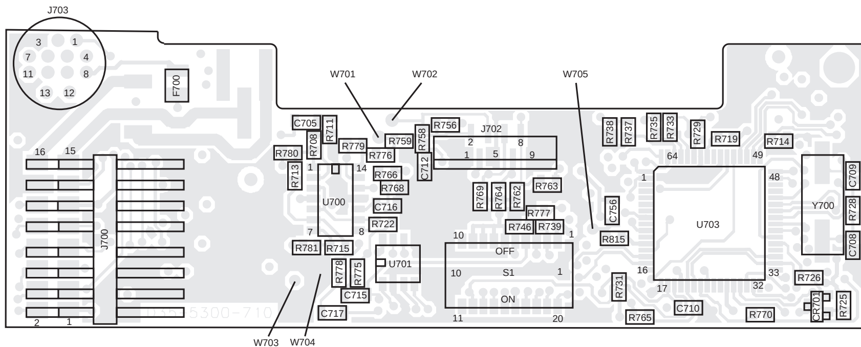
TOP VIEW
