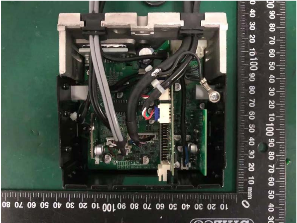
Internal Photos M/N: Motor 4
