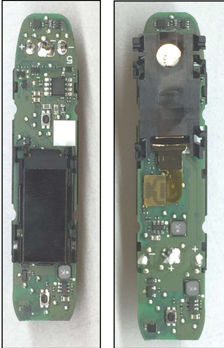
Main board with display
