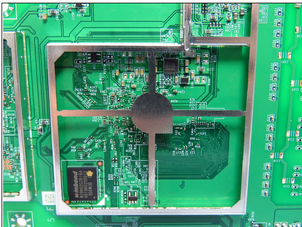
Mode 1: 1 st 2.4G FEM
