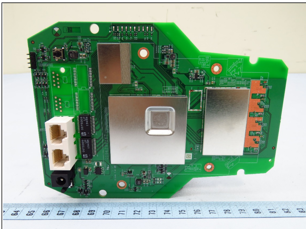
Option A: PCB without absorber
