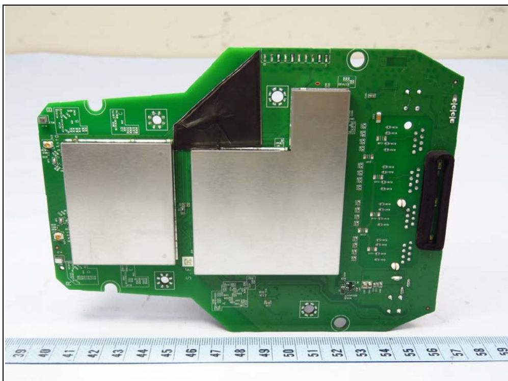
Option C: PCB with absorber
