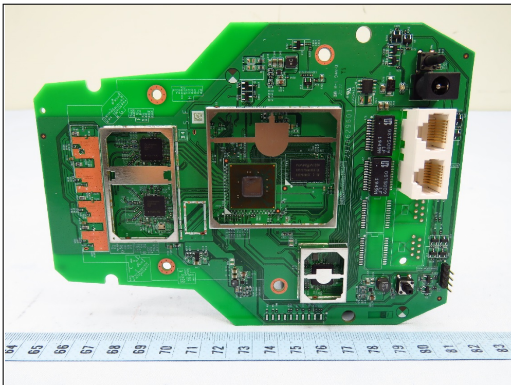
Option B: PCB with absorber
