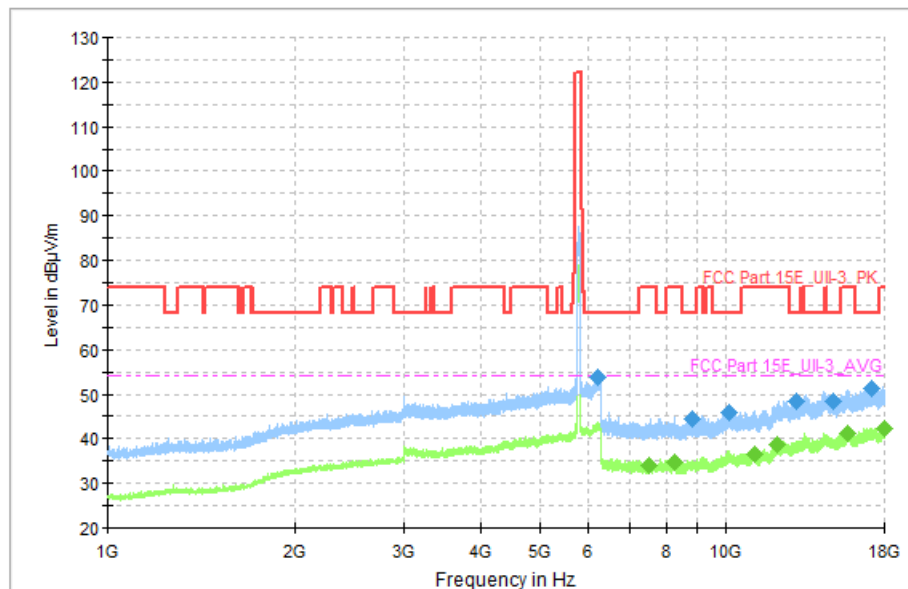
Fig. 65 Transmitter Spurious Emission (802. 11ac-VHT80, CH155 5775MHz)
