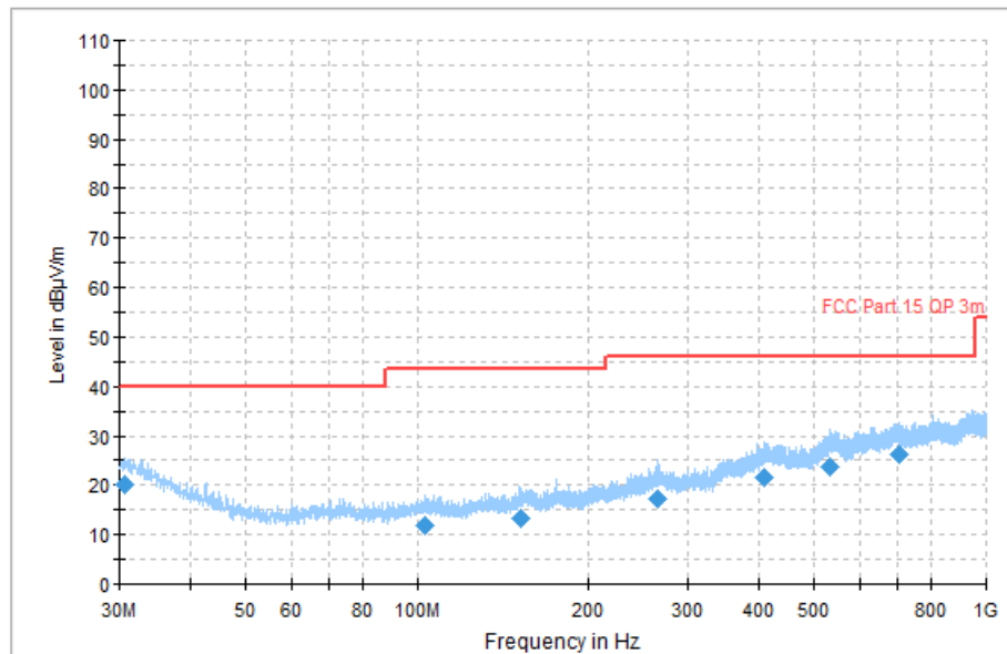
Fig. 66 Transmitter Spurious Emission (All channel, 30MHz~1GHz)
