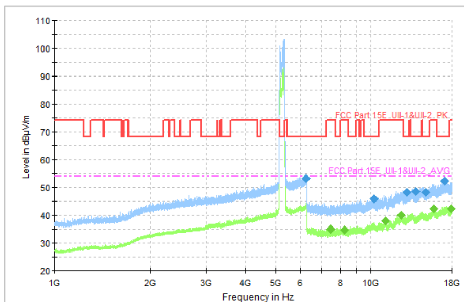
Fig. 59 Transmitter Spurious Emission (802.11n-HT40, CH54 5270MHz)
