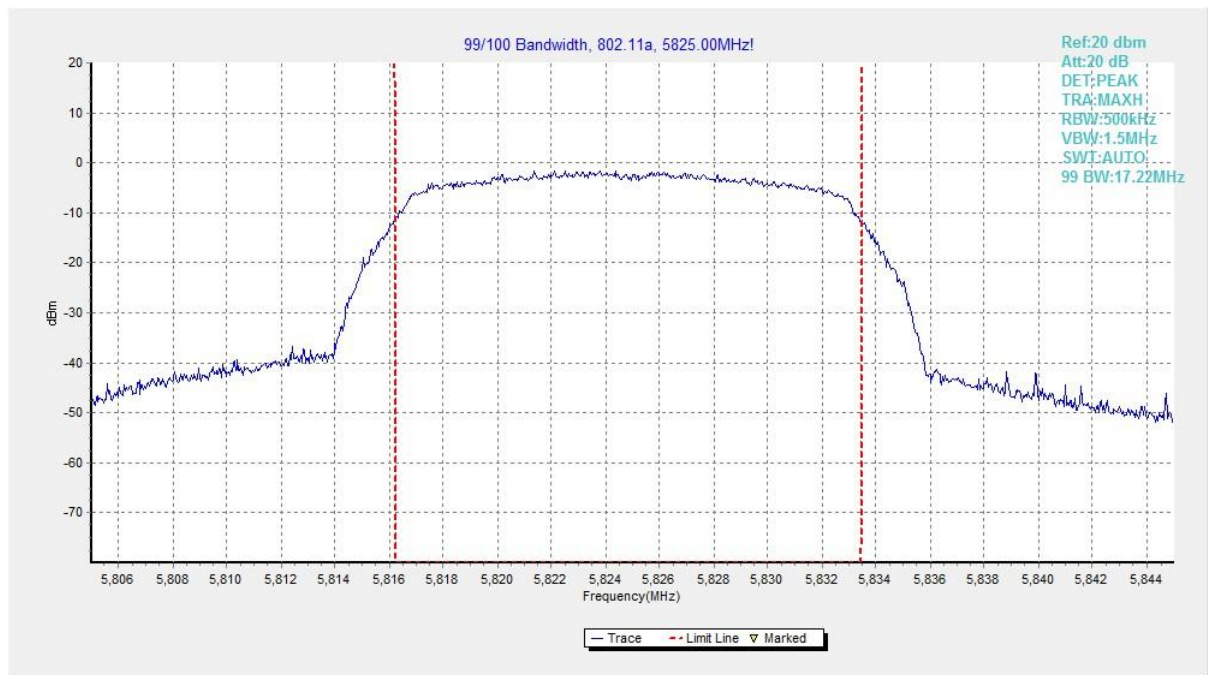
Fig. 27 99% Occupied Bandwidth (802.11a, 5825MHz)
