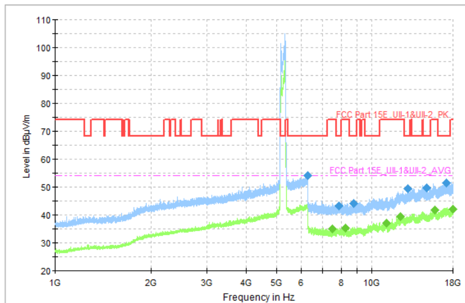
Fig. 64 Transmitter Spurious Emission (802. 11ac-VHT80, CH58 5290MHz)
