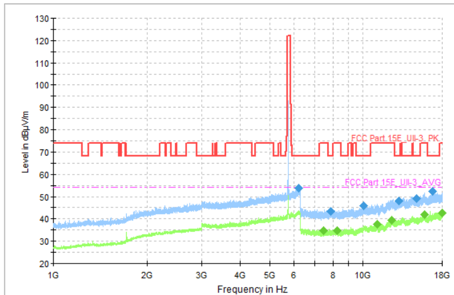
Fig. 54 Transmitter Spurious Emission (802. 11a, CH149 5745MHz)
