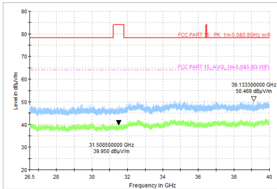
Fig. 68 Transmitter Spurious Emission (All channel, 26.5GHz~40GHz)
