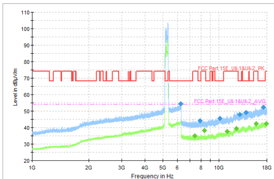
Fig. 58 Transmitter Spurious Emission (802.11n-HT40, CH46 5230MHz)
