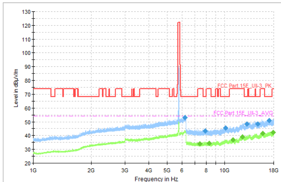
Fig. 61 Transmitter Spurious Emission (802. 11n-HT40, CH151 5755MHz)
