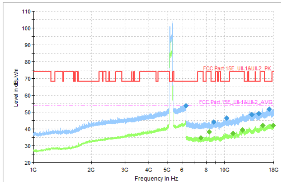
Fig. 60 Transmitter Spurious Emission (802.11n-HT40, CH62 5310MHz)
