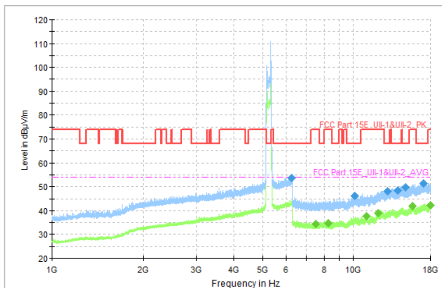
Fig. 53 Transmitter Spurious Emission (802.11a, CH64 5320MHz)
