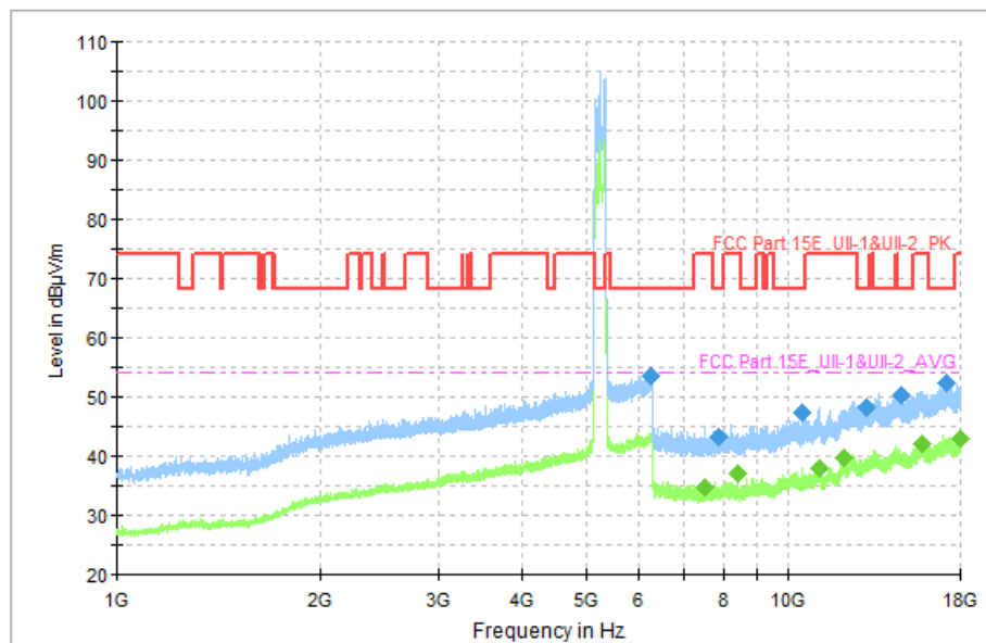
Fig. 50 Transmitter Spurious Emission (802.11a, CH48 5240MHz)
