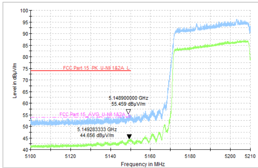
Fig. 45 Band Edges (802.11ac-VHT80, CH42 5210MHz)
