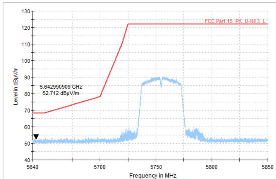
Fig. 43 Band Edges (802.11n-HT40, CH151 5755MHz)
