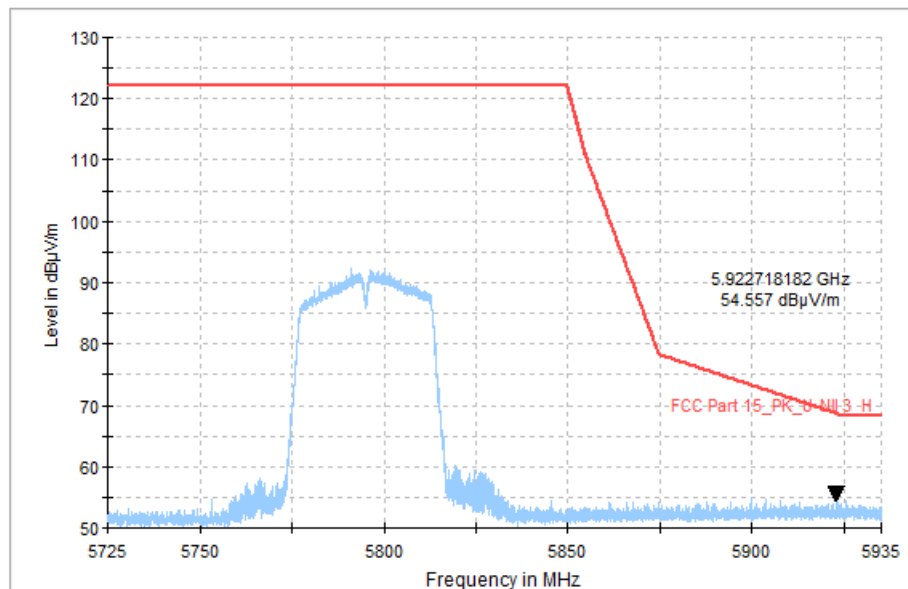
Fig. 44 Band Edges (802.11n-HT40, CH159 5795MHz)
