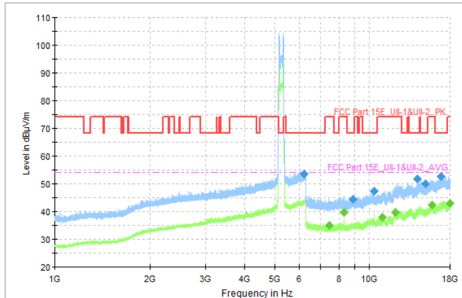
Fig. 48 Transmitter Spurious Emission (802.11a, CH36 5180MHz)
