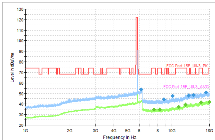
Fig. 56 Transmitter Spurious Emission (802.11a, CH165 5825MHz)
