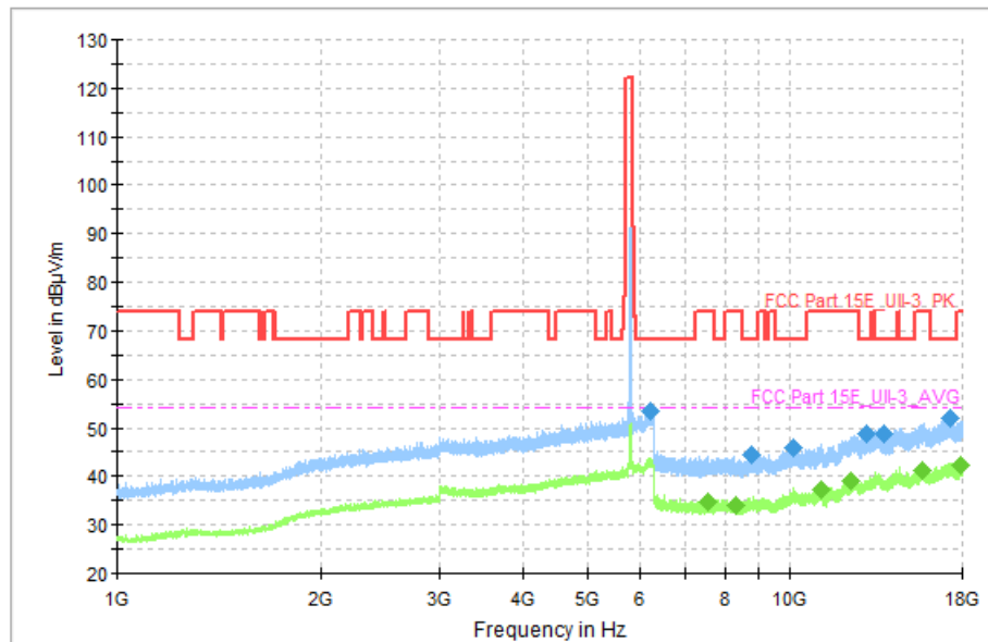
Fig. 62 Transmitter Spurious Emission (802. 11n-HT40, CH159 5795MHz)
