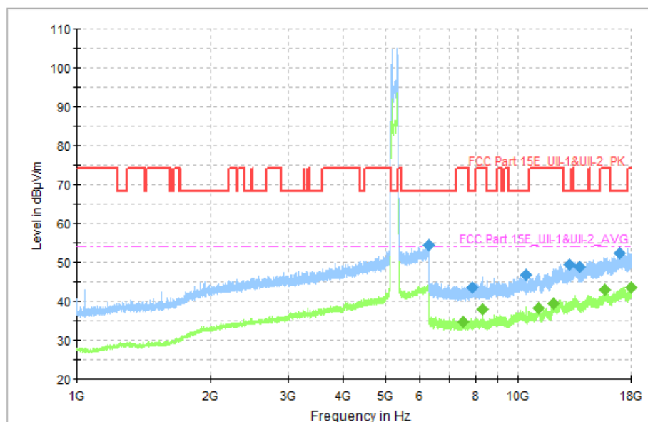
Fig. 49 Transmitter Spurious Emission (802.11a, CH40 5200MHz)
