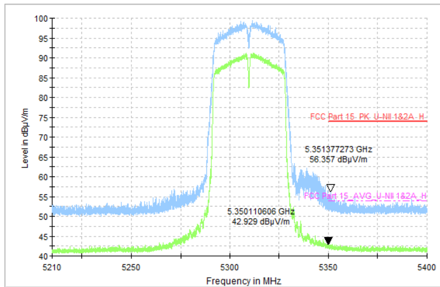
Fig. 42 Band Edges (802.11n-HT40, CH62 5310MHz)
