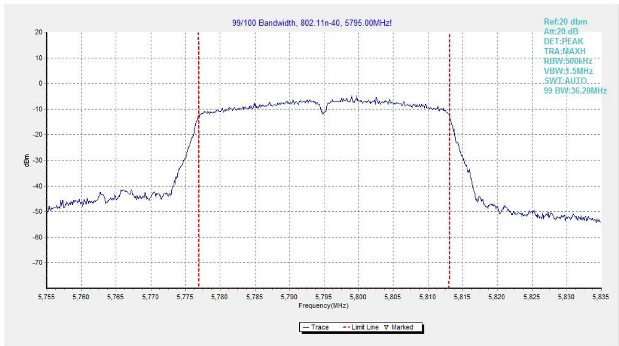
Fig. 33 99% Occupied Bandwidth (802.11n-HT40, 5795MHz)
