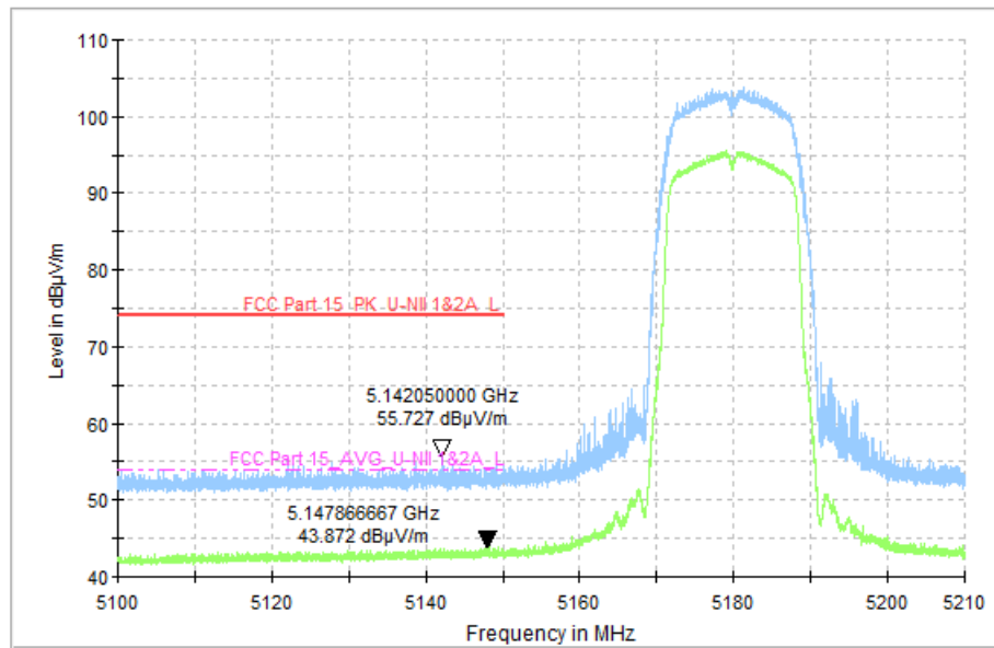
Fig. 37 Band Edges (802.11a, CH36 5180MHz)
