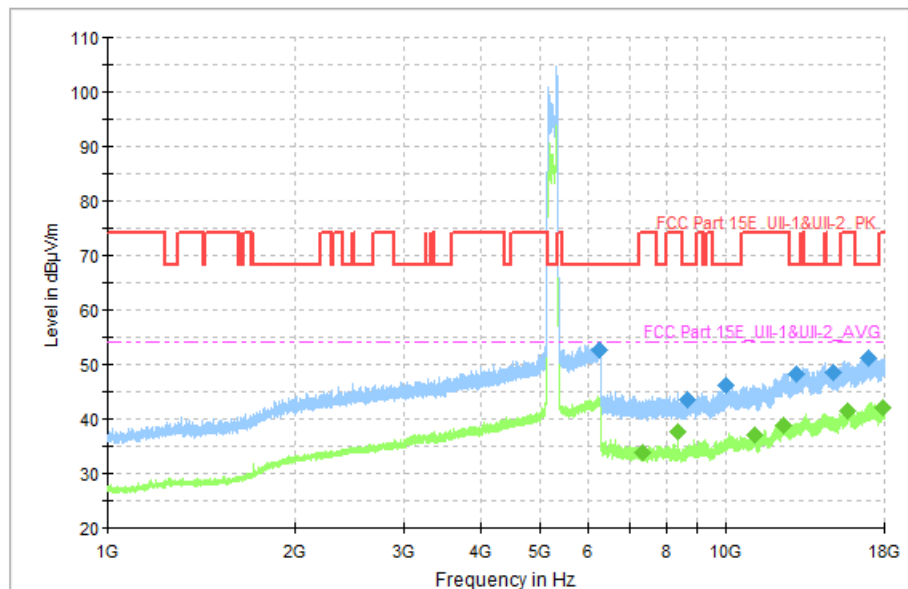
Fig. 63 Transmitter Spurious Emission (802. 11ac-VHT80, CH42 5210MHz)
