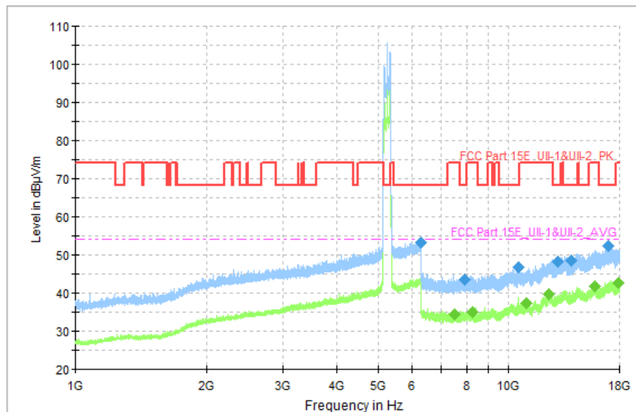
Fig. 51 Transmitter Spurious Emission (802.11a, CH52 5260MHz)
