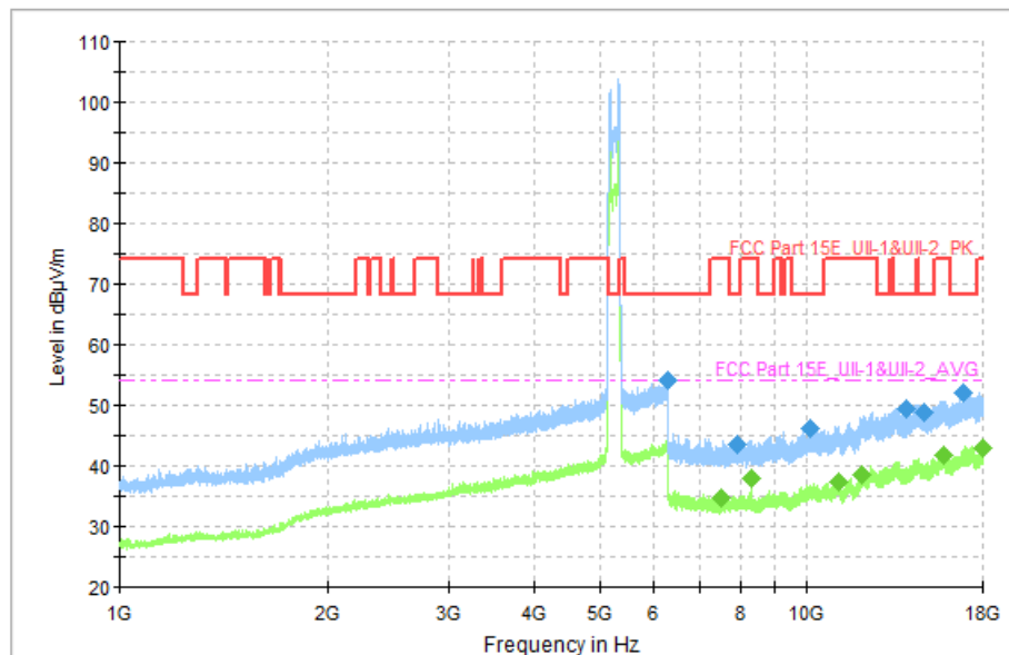
Fig. 57 Transmitter Spurious Emission (802.11n-HT40, CH38 5190MHz)
