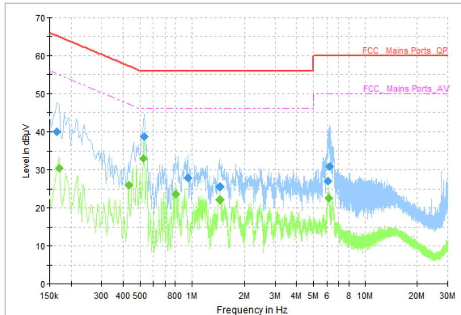
Fig. 73 AC Power line Conducted Emission (Idle)
