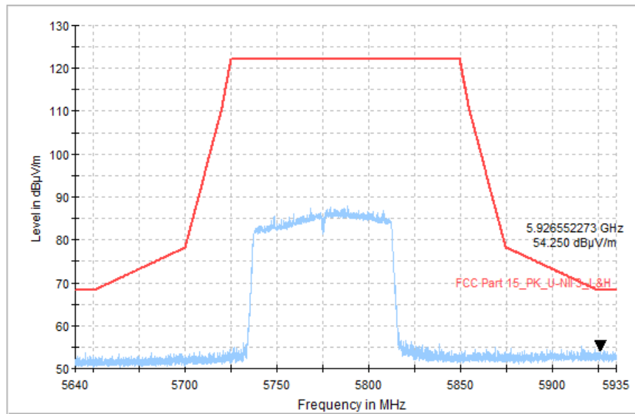
Fig. 47 Band Edges (802.11ac-VHT80, CH155 5775MHz)
