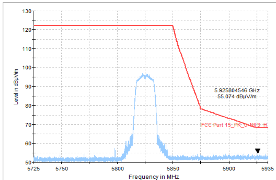
Fig. 40 Band Edges (802.11a, CH165 5825MHz)
