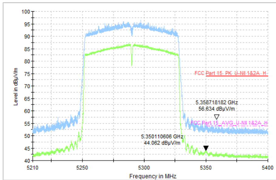
Fig. 46 Band Edges (802.11ac-VHT80, CH58 5290MHz)
