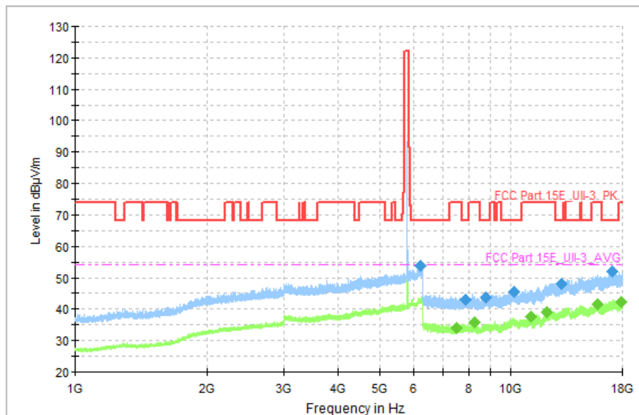
Fig. 55 Transmitter Spurious Emission (802. 11a, CH157 5785MHz)
