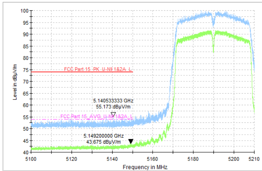
Fig. 41 Band Edges (802.11n-HT40, CH38 5190MHz)
