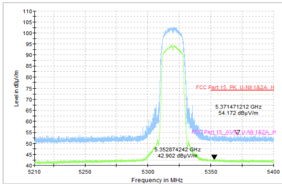
Fig. 38 Band Edges (802.11a, CH64 5320MHz)
