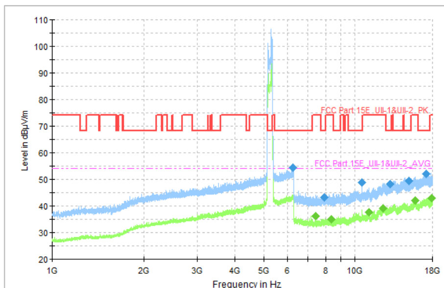
Fig. 52 Transmitter Spurious Emission (802.11a, CH56 5280MHz)
