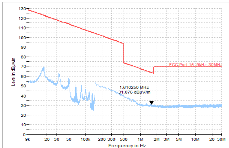
Fig. 69 Radiated Spurious Emission (All Channel, 9 kHz ~ 30 MHz)
