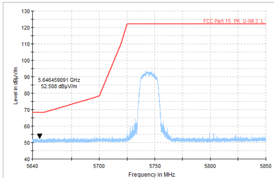
Fig. 39 Band Edges (802.11a, CH149 5745MHz)
