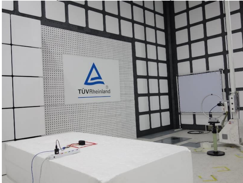
Photograph 3: Test Setup for Spurious Emissions (Back View 1)
