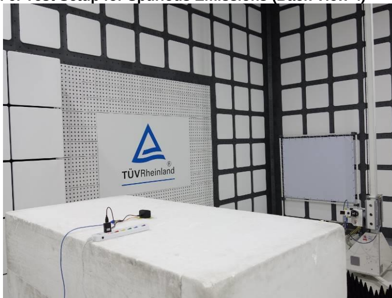
Photograph 6: Test Setup for Spurious Emissions (Back View 4)
