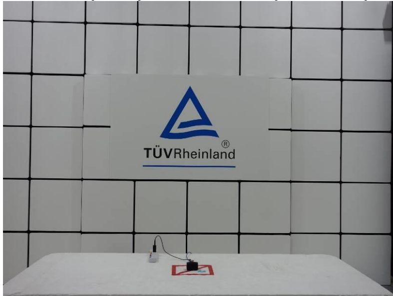
Photograph 1: Test Setup for Spurious Emissions (Front View 1)
